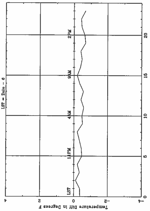
Average Diurnal Cycle for ISN - fall
