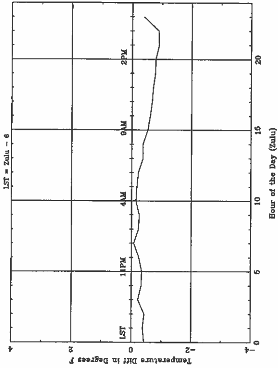
Average Diurnal Cycle for MCI - winter
