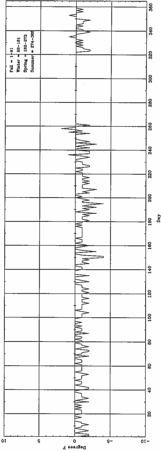
Daily \Delta T (highest buoy) (ASOS - CONV) for APN
