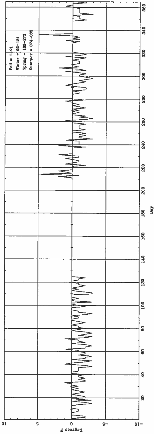
Daily \Delta T_{(light\ hour)} (ASOS - CONV) for TRI
