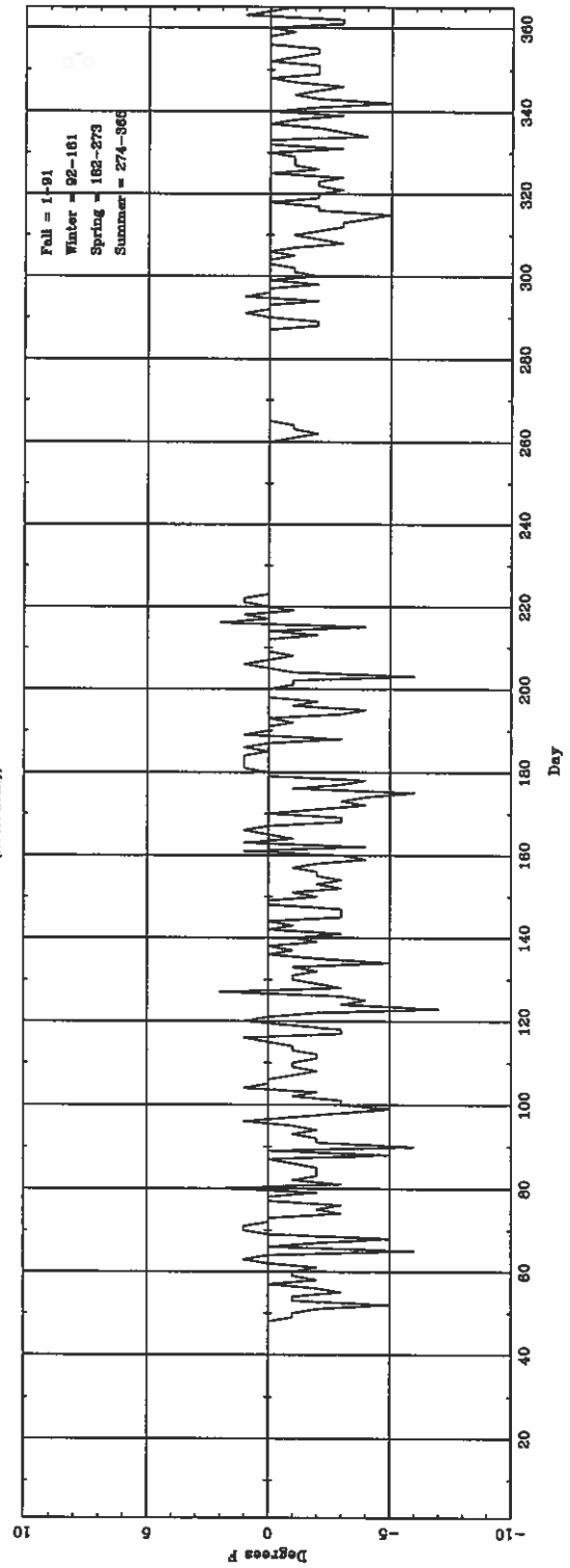
Daily \Delta T_{\text{[lowest hourly]}} (ASOS - CONY) for LBF
