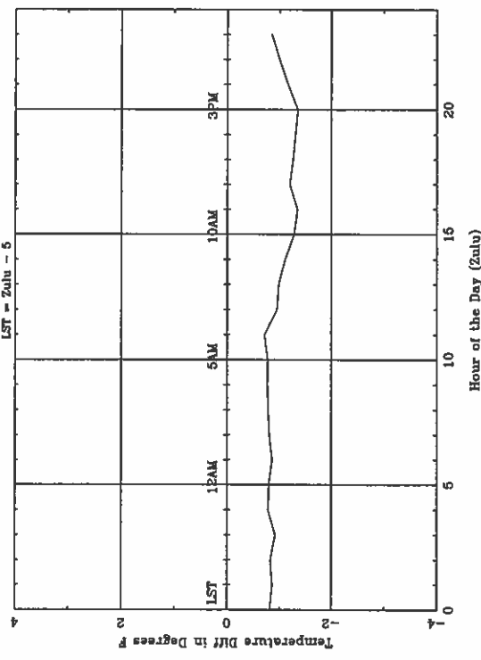
Average Diurnal Cycle for DTW - fall
