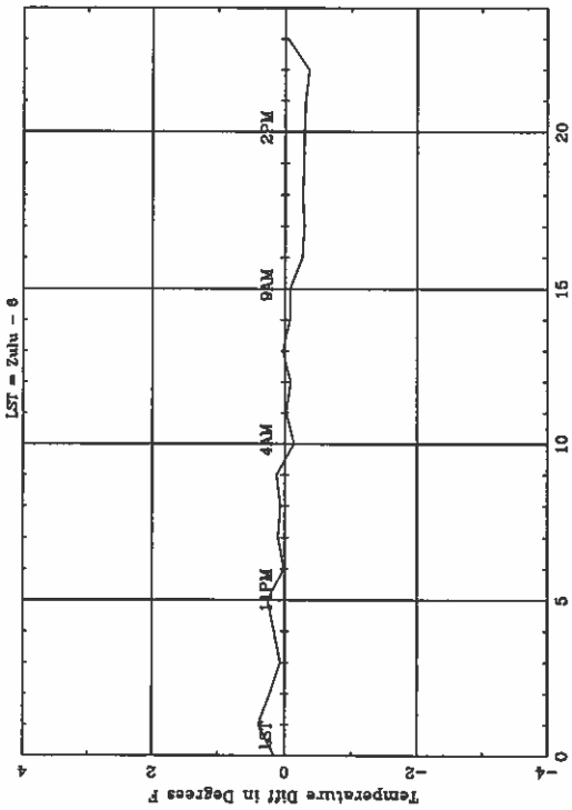
Average Diurnal Cycle for RST - fall
