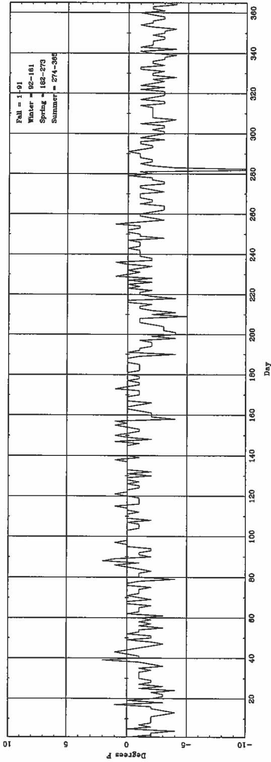
Daily \Delta T_{\text{(lightest hourly)}} (ASOS - CONV) for JKL
