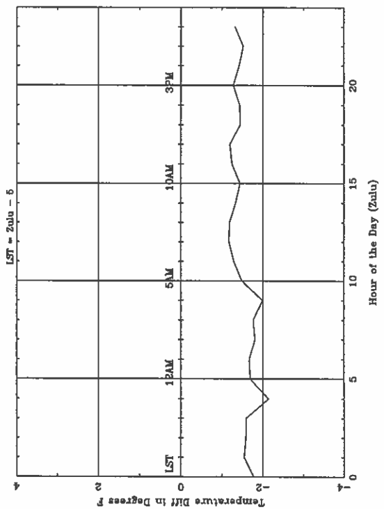
Average Diurnal Cycle for ABE - spring
