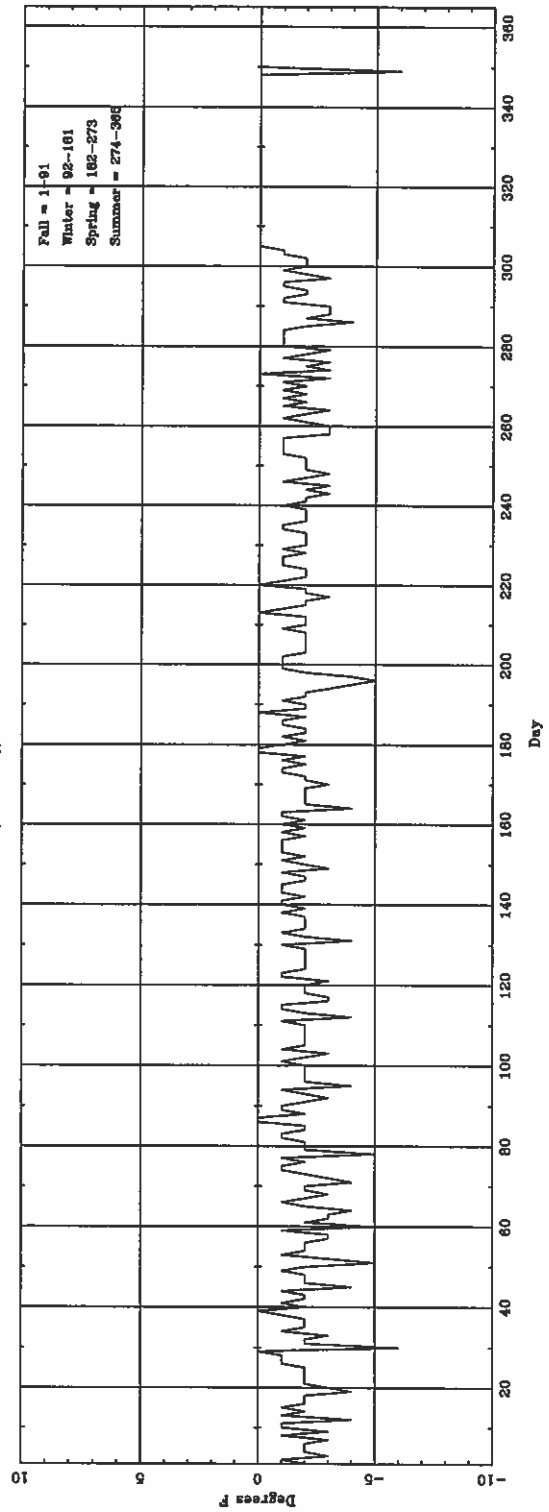
Daily \Delta T_{\text{freshest beauty}} (ASOS - CONV) for MKE
