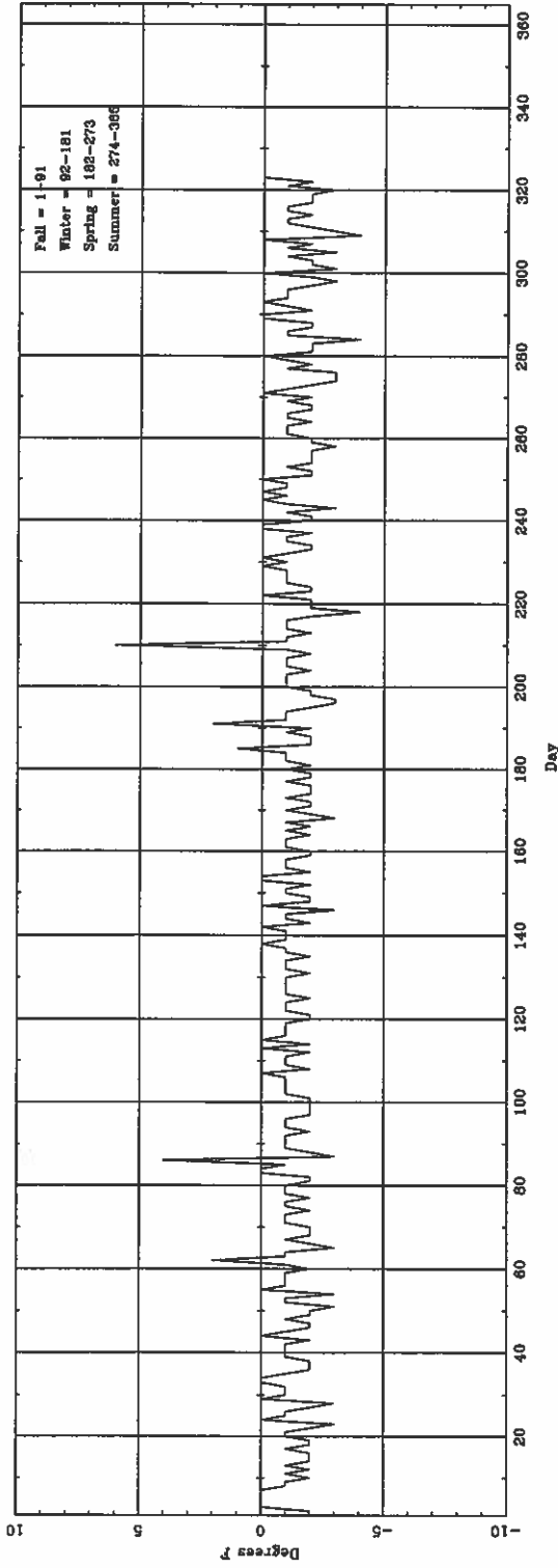
Daily \Delta T_{(highest\ hourly)} (ASOS - CONV) for LCH
