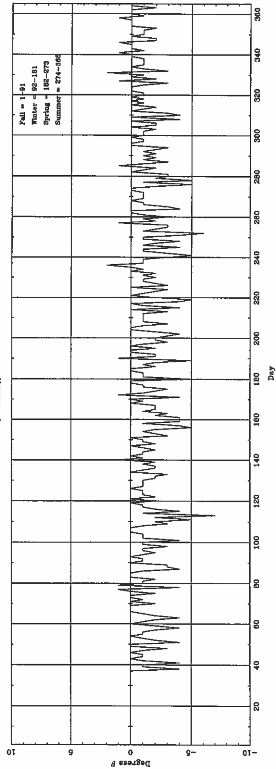
Daily AT (overcast hourly) (ASOS - CONV) for ABQ
