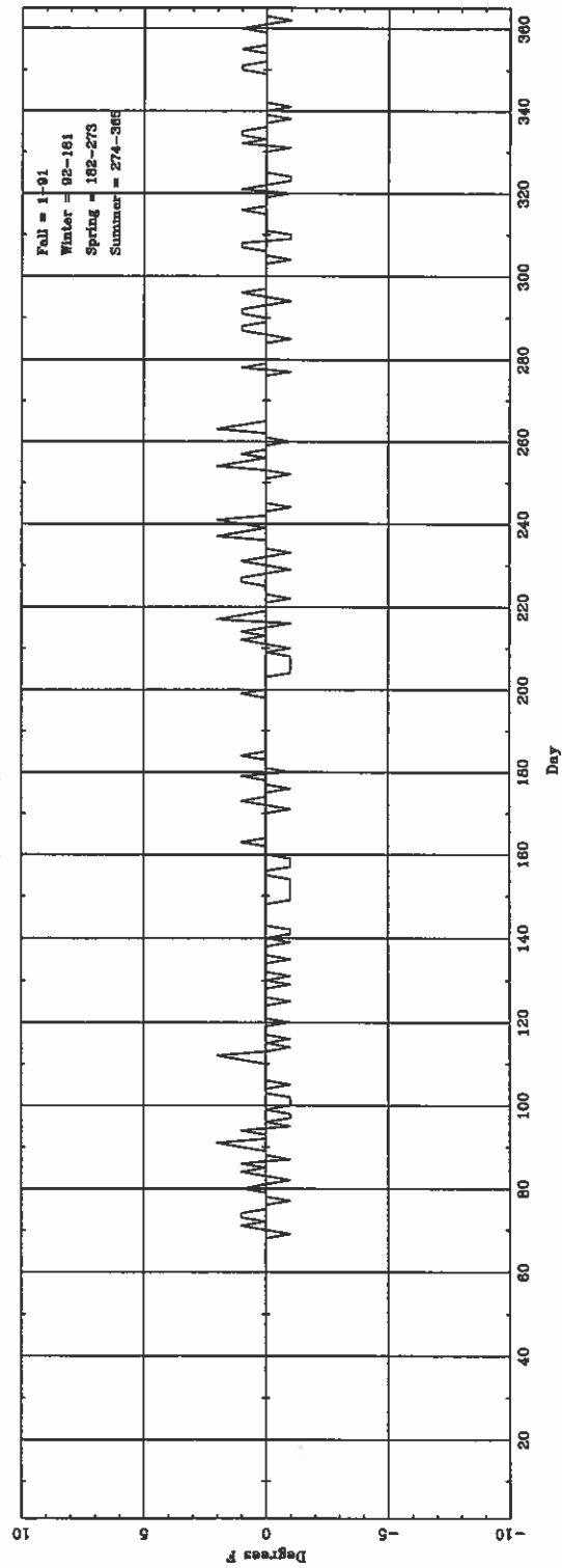
Daily \Delta T_{(forest\ beam)} (ASOS - CONV) for DAY
