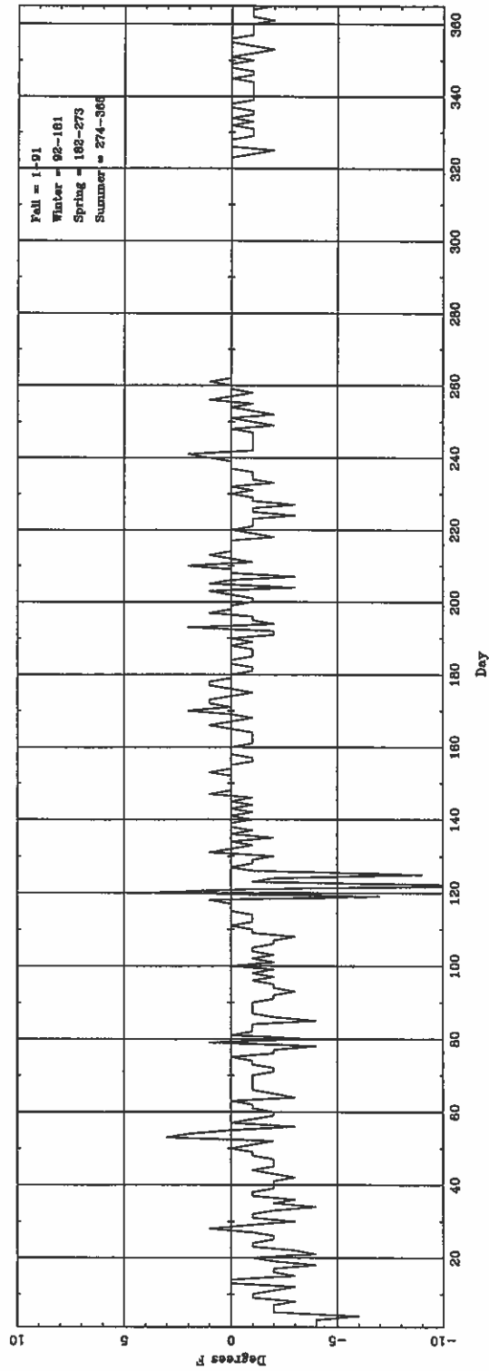
Daily AT (fourest hourly) (ASOS - CONV) for FWA
