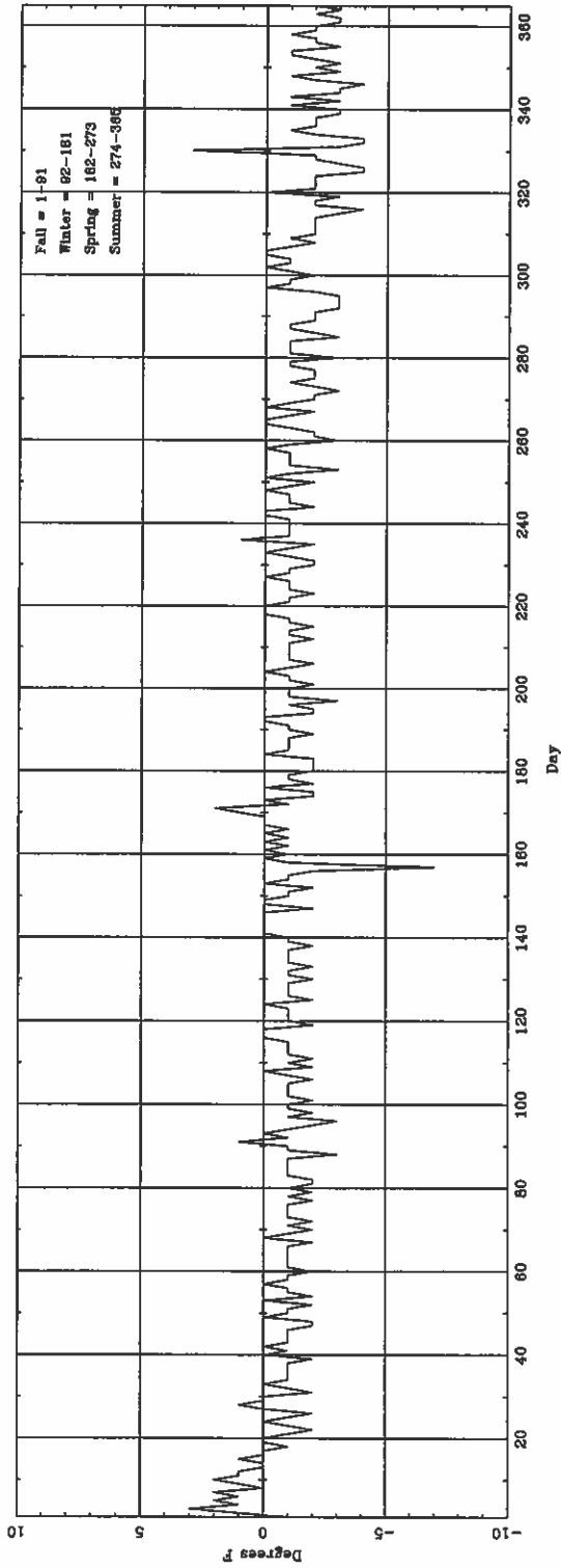
Daily \Delta T (adjusted hourly) (ASOS - CONV) for DSM
