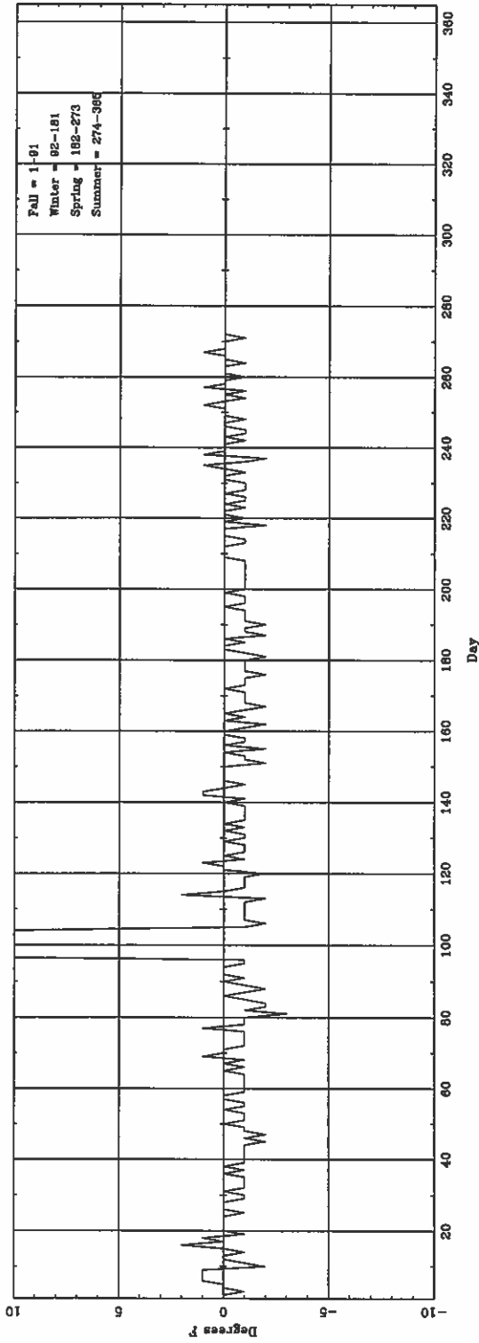
Daily AT (subject hourly) (ASOS - CONY) for PDT
