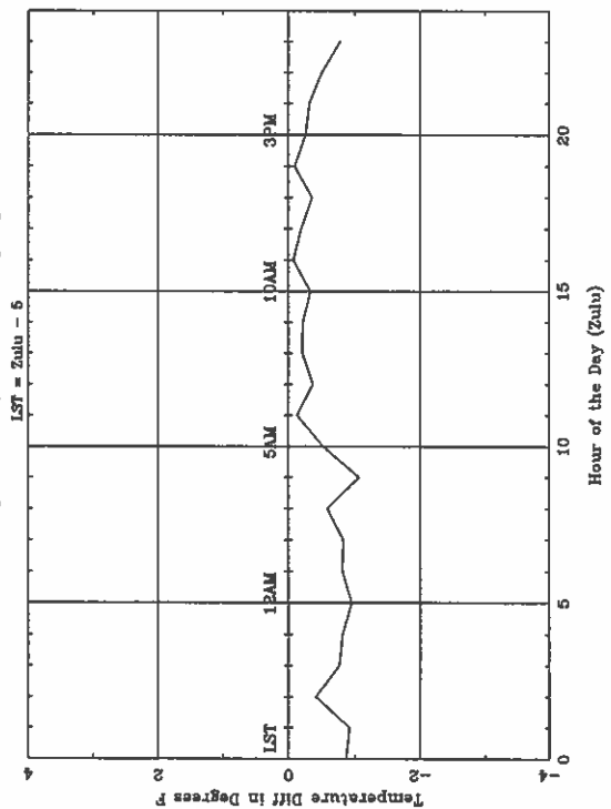
Average Diurnal Cycle for ACY - spring
