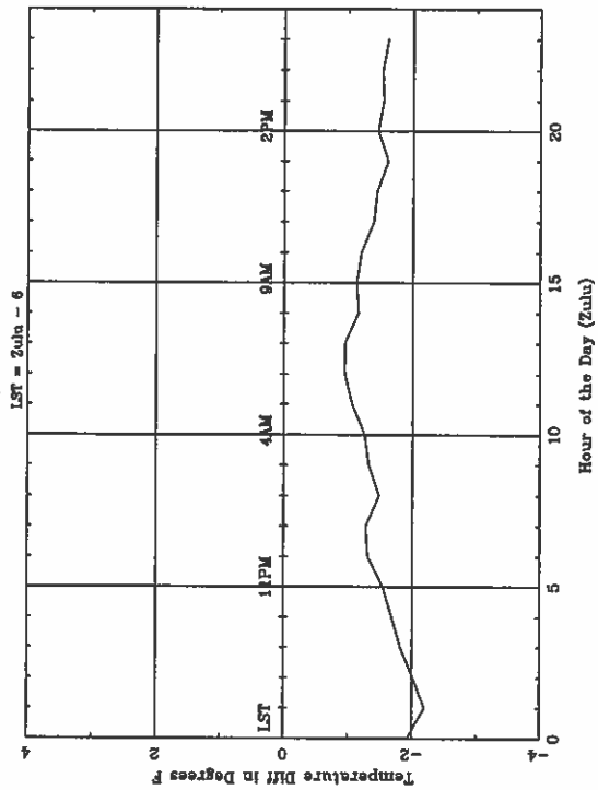
Average Diurnal Cycle for SPI - summer
