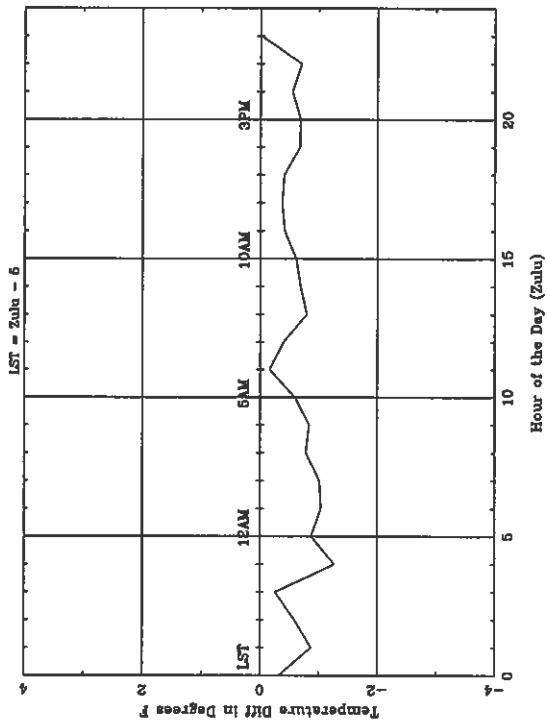
Average Diurnal Cycle for TRI - summer
