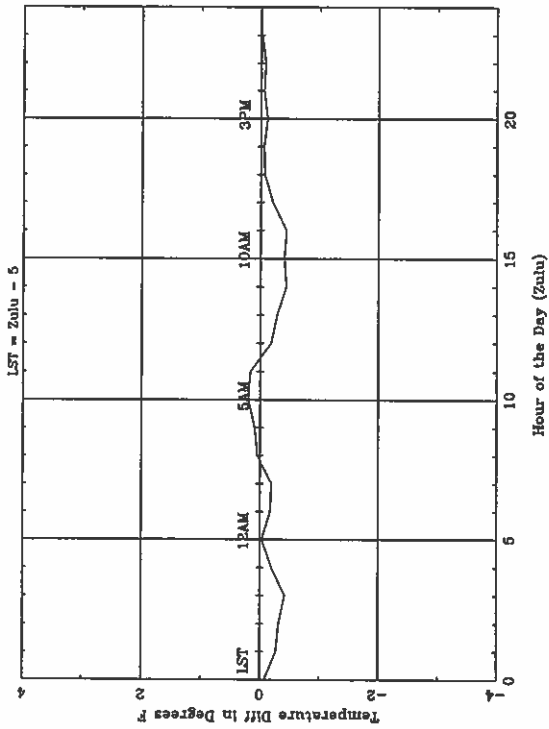
Average Diurnal Cycle for DAB - fall
