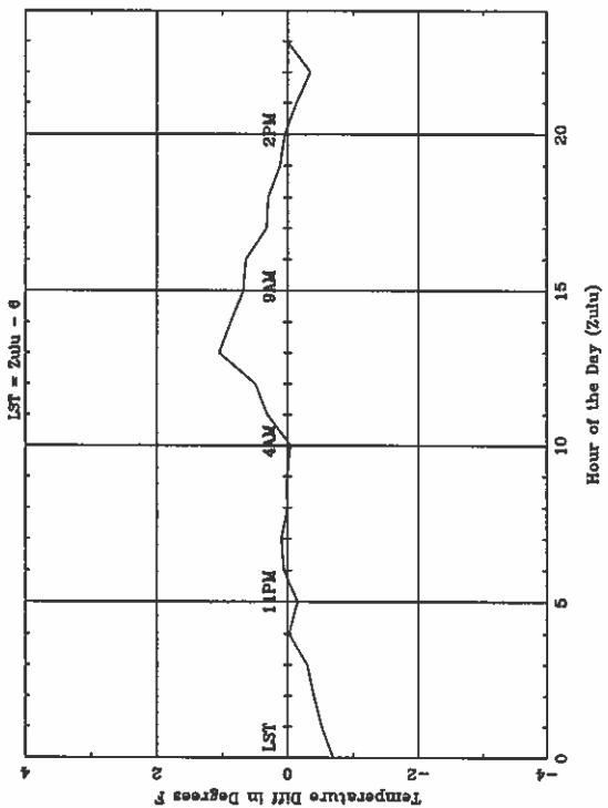
Average Diurnal Cycle for VTN - spring
