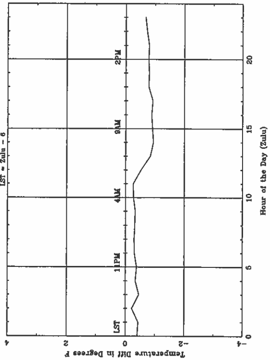
Average Diurnal Cycle for MOB - summer LST = Zulu - 6
