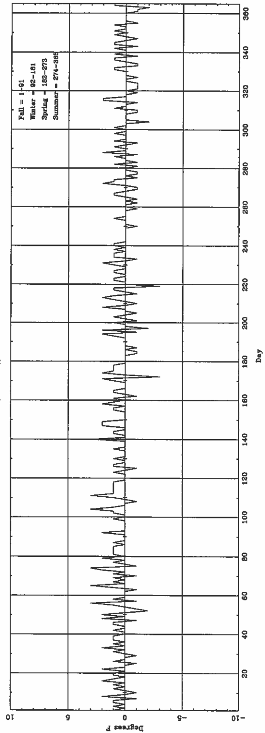
Daily \Delta T_{\text{(foremost hourly)}} (ASOS - CONV) for JKL
