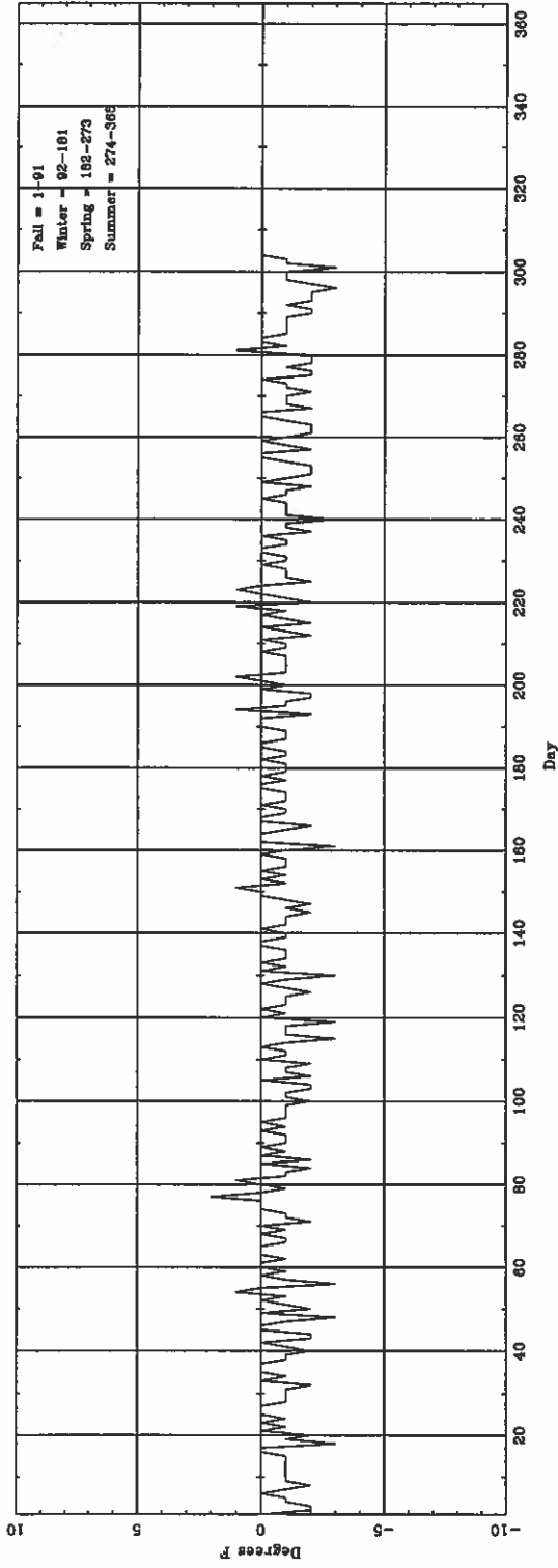
Daily \Delta T_{(highest\ hourly)} (ASOS - CONV) for MCI
