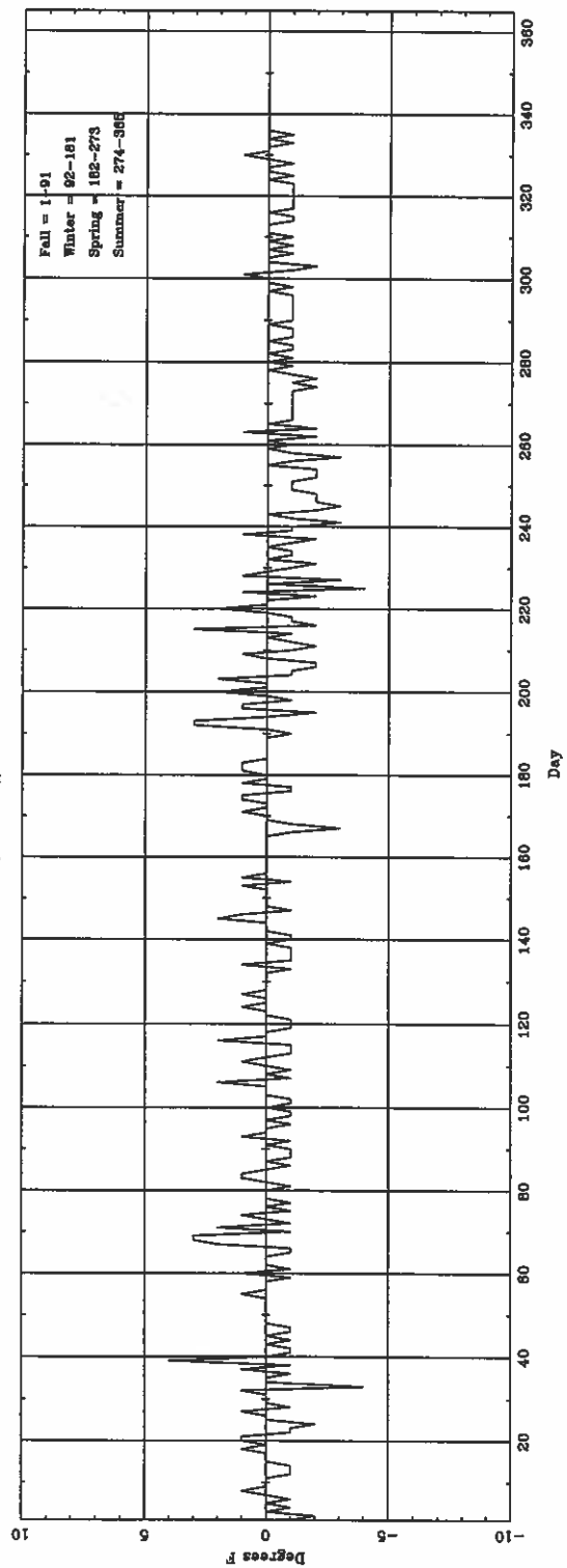
Daily \Delta T_{\text{(warmest hourly)}} (ASOS -- CONY) for PAH
