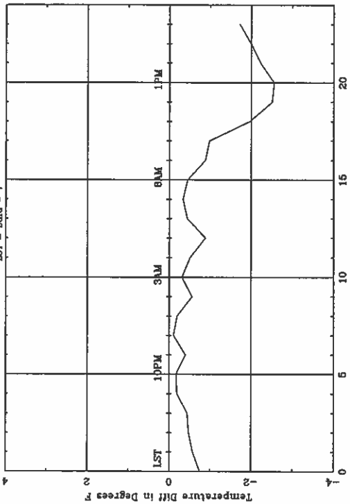
Average Diurnal Cycle for TUS - fall LST = Zulu - 7
