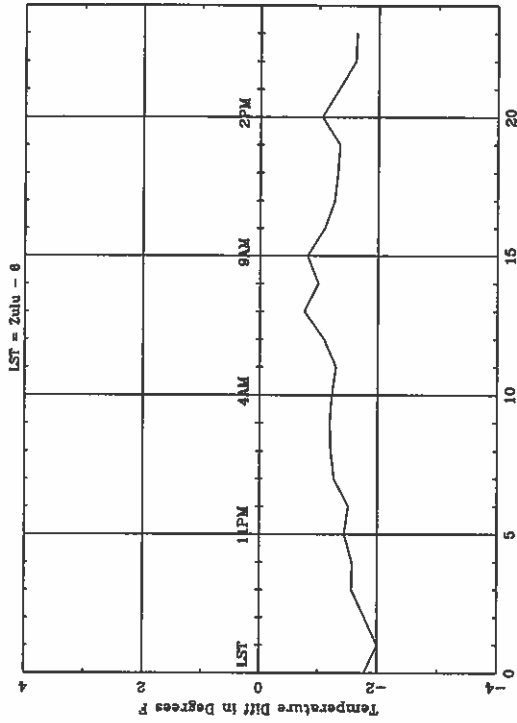
Average Diurnal Cycle for LCH - winter
