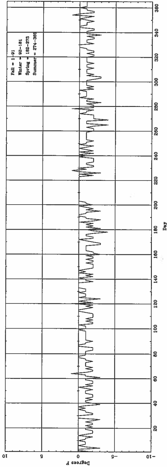
Daily AT (August hourly) (ASOS - CONV) for LAS
