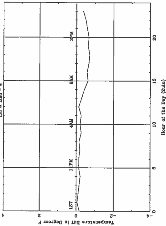
Average Diurnal Cycle for MOB - fall LST = Zulu - 6
