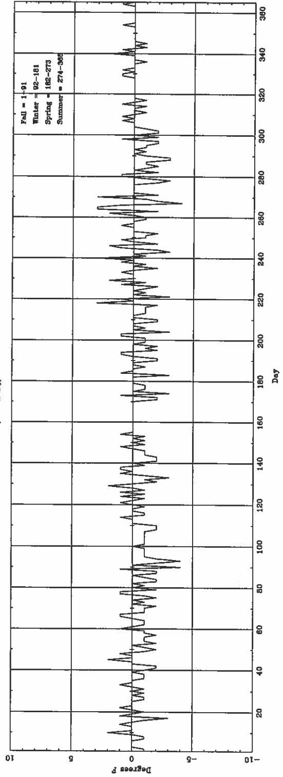
Daily \Delta T_{(warmest\ hour)} (ASOS - CONV) for TUS
