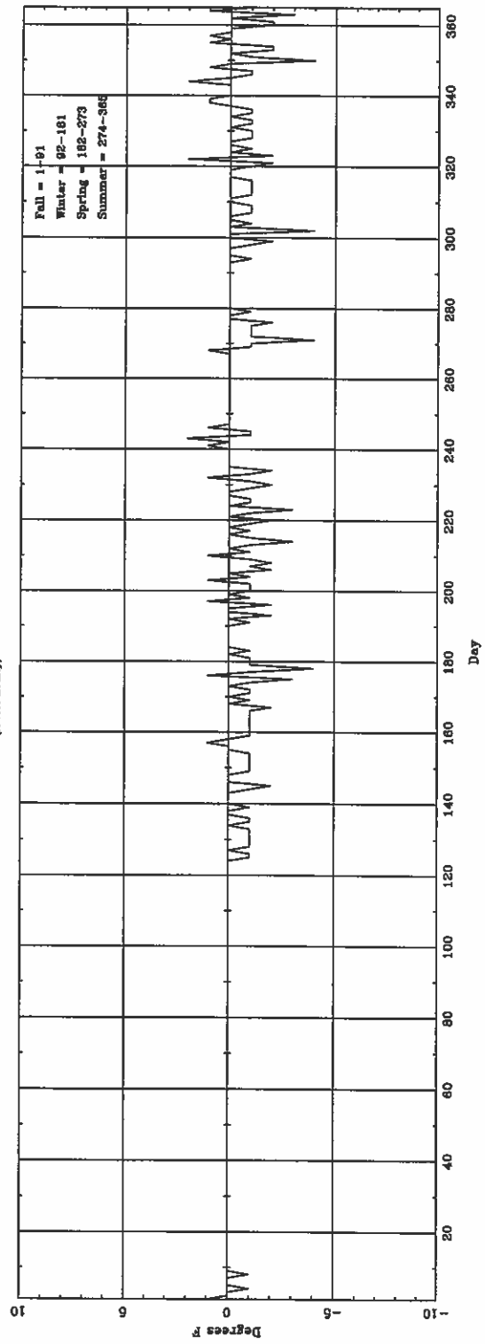
Daily \Delta T (lowest hourly) (ASOS - CONV) for GEG
