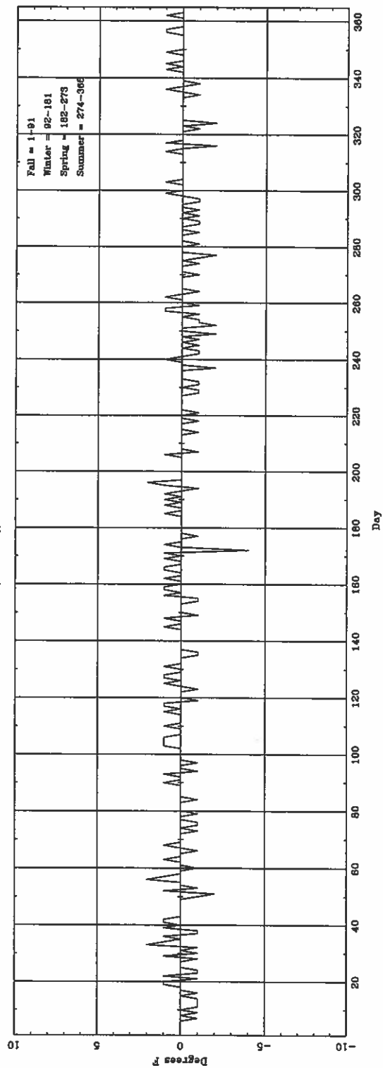
Daily \Delta T_{(night\ hour)} (ASOS - CONV) for LEX
