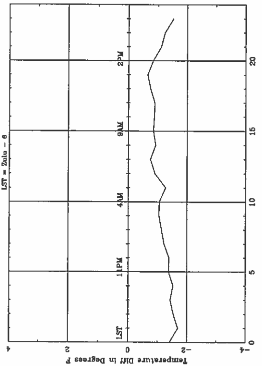
Average Diurnal Cycle for SPI - fall
