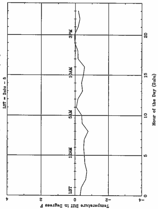
Average Diurnal Cycle for DAB - spring
