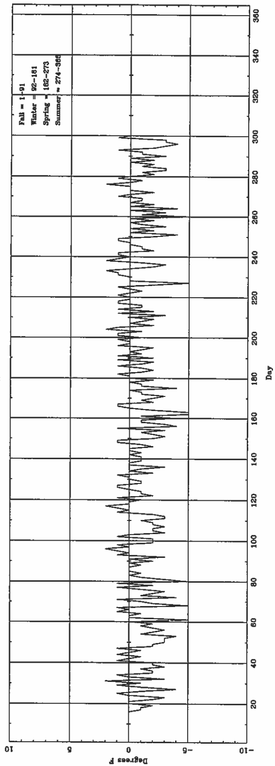
Daily AT (correct hourly) (ASOS - CONV) for INW
