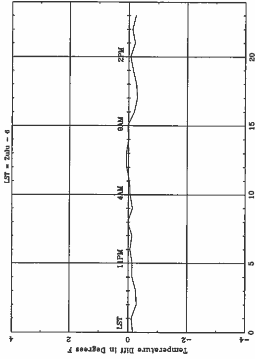
Average Diurnal Cycle for RST - winter
