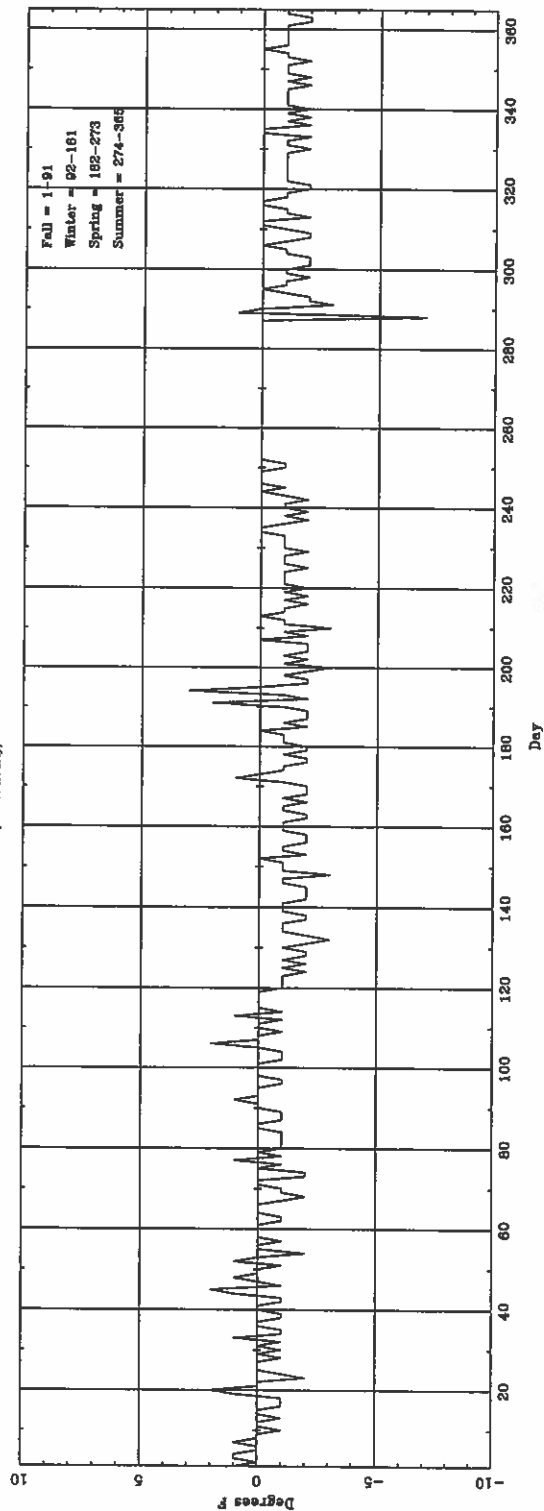
Daily \Delta T_{(current\ hourly)} (ASOS - CONV) for YNG
