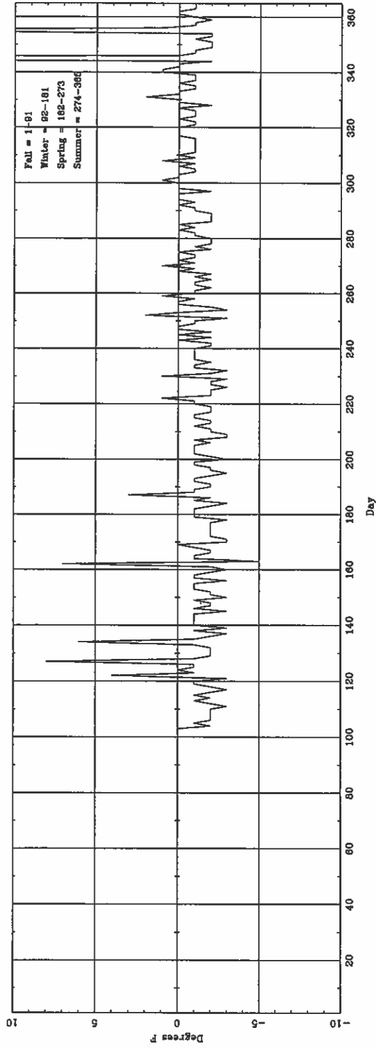
Daily \Delta T_{(\text{largest hourly})} (ASOS - CONY) for ABE
