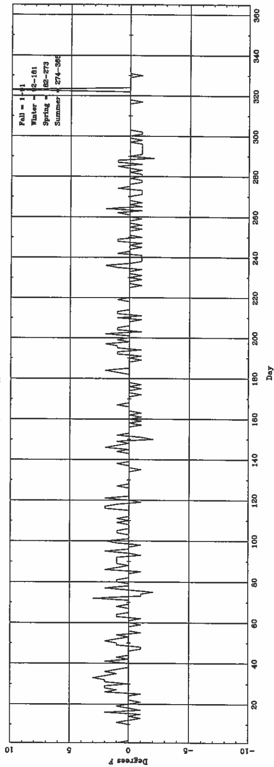
Daily \Delta T (nearest hourly) (ASOS - CONY) for RFD
