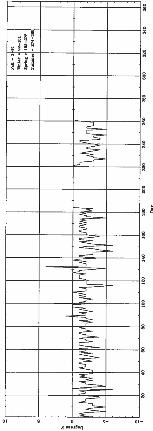
Daily \Delta T (coldest hourly) (ASOS - CONV) for MSN
