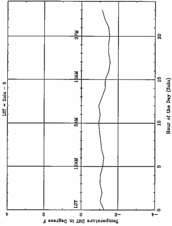
Average Diurnal Cycle for YNG - winter
