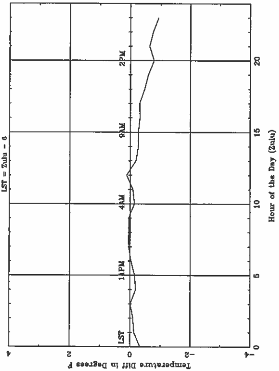
Average Diurnal Cycle for MCI - fall
