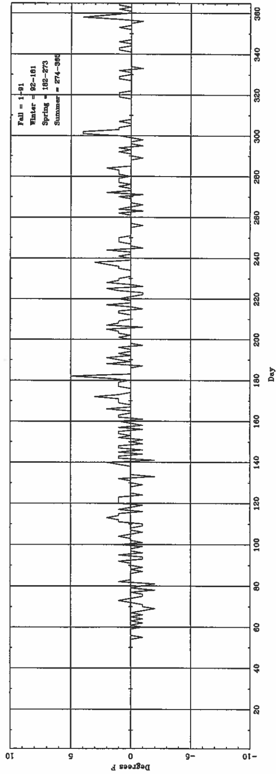
Daily \Delta T_{(normal\ hourly)} (ASOS - CONV) for PDX
