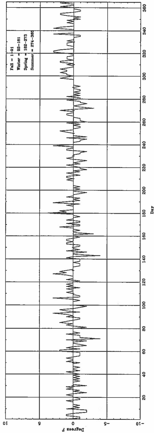
Daily AT (August hourly) (ASOS - CONV) for BIS
