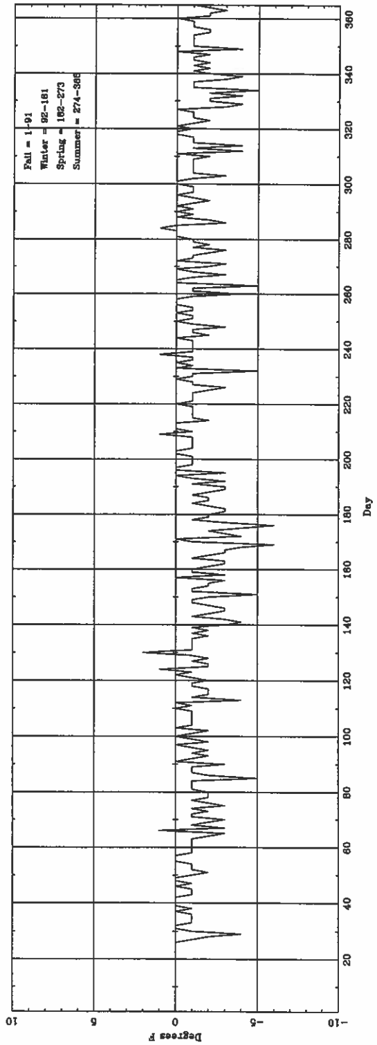
Daily \Delta T (lowest hourly) (ASOS - CONV) for FAR
