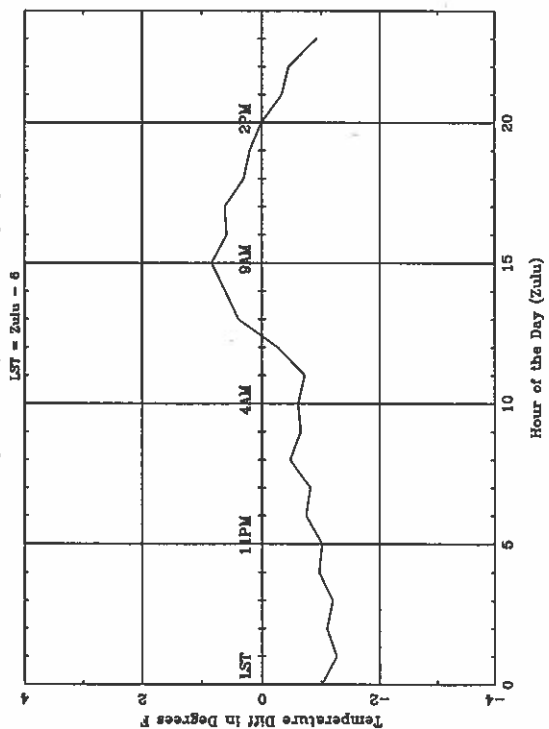
Average Diurnal Cycle for SLN - spring
