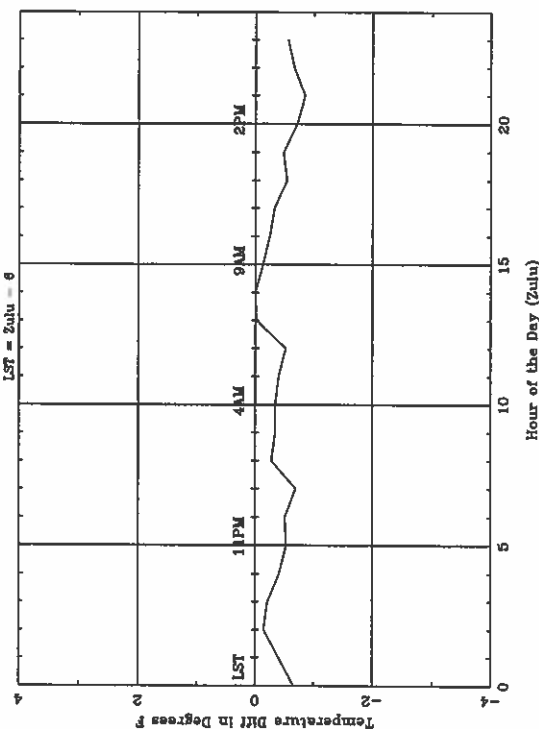
Average Diurnal Cycle for LBF - spring
