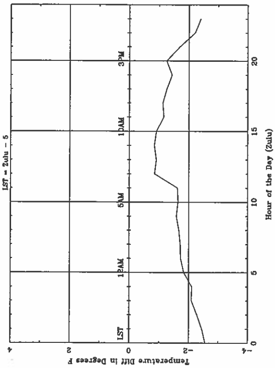
Average Diurnal Cycle for SAV - fall
