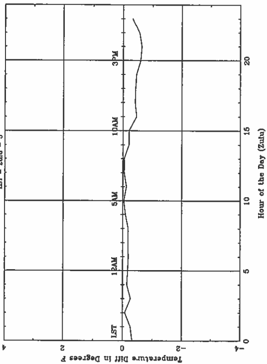
Average Diurnal Cycle for MKG - fall LST = Zulu - 5
