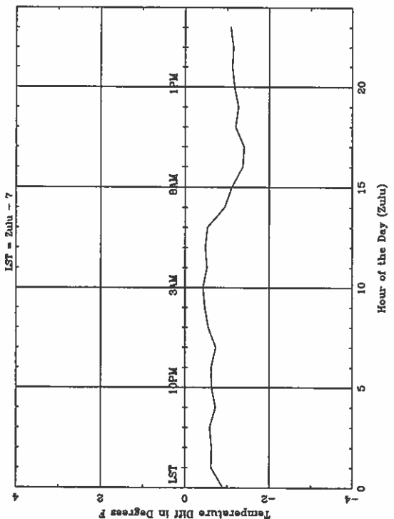
Average Diurnal Cycle for CYS - spring
