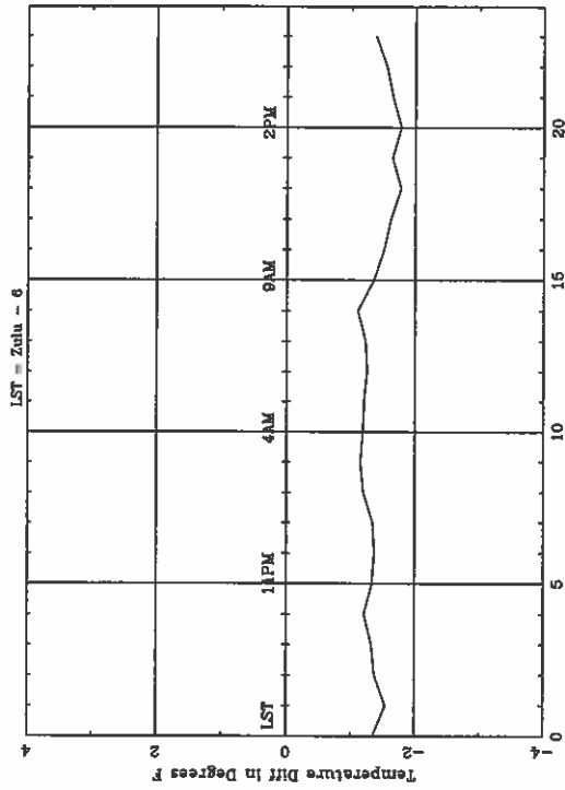
Average Diurnal Cycle for FAR - winter
