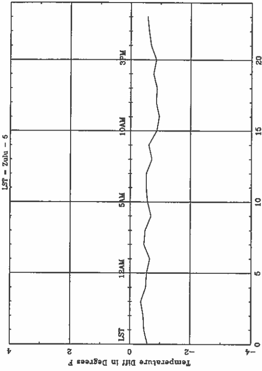
Average Diurnal Cycle for BGM - winter
