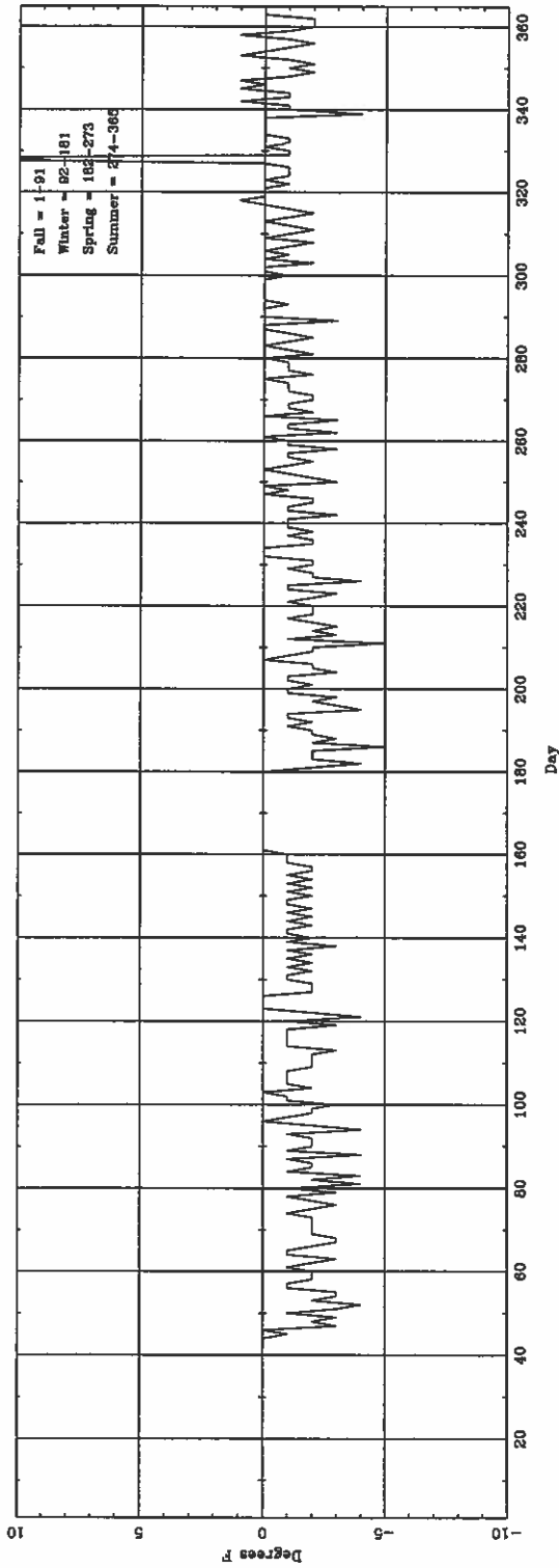
Daily \Delta T_{\text{surface buoy}} (ASOS - CONV) for EUG
