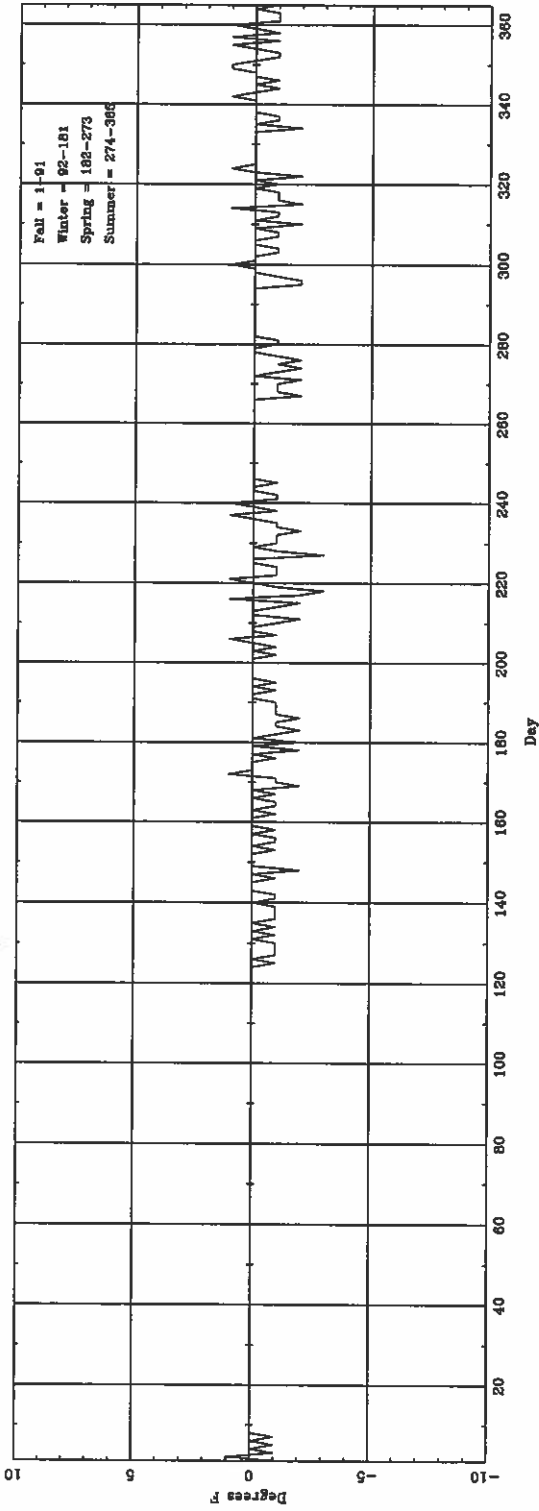
Daily \Delta T (lightest hourly) (ASOS - CONV) for GRG
