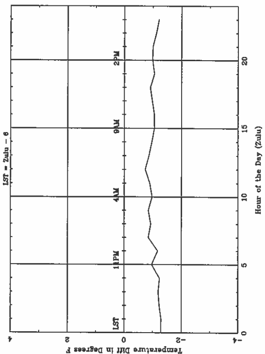
Average Diurnal Cycle for SPI - spring
