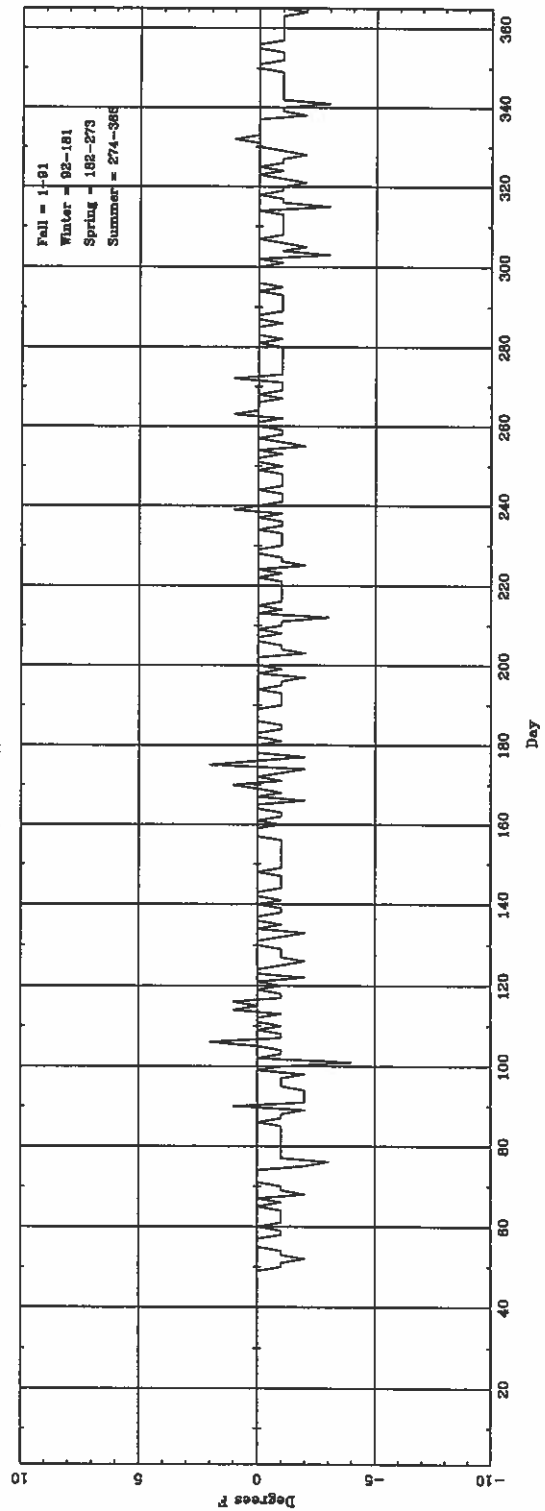
Daily \Delta T_{\text{lowest hourly}} (ASOS - CONV) for OFK
