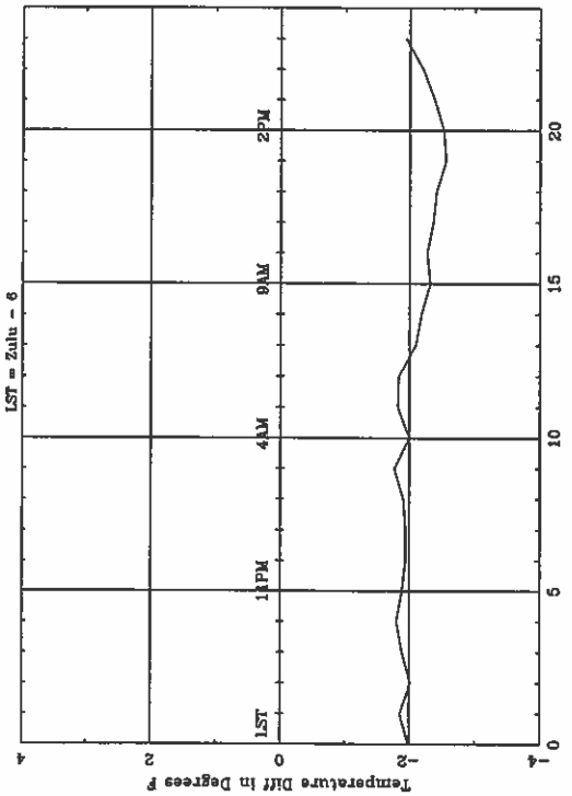
Average Diurnal Cycle for MKE - fall
