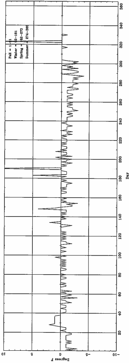
Daily \Delta T (highest hourly) (ASOS - CONY) for RFD
