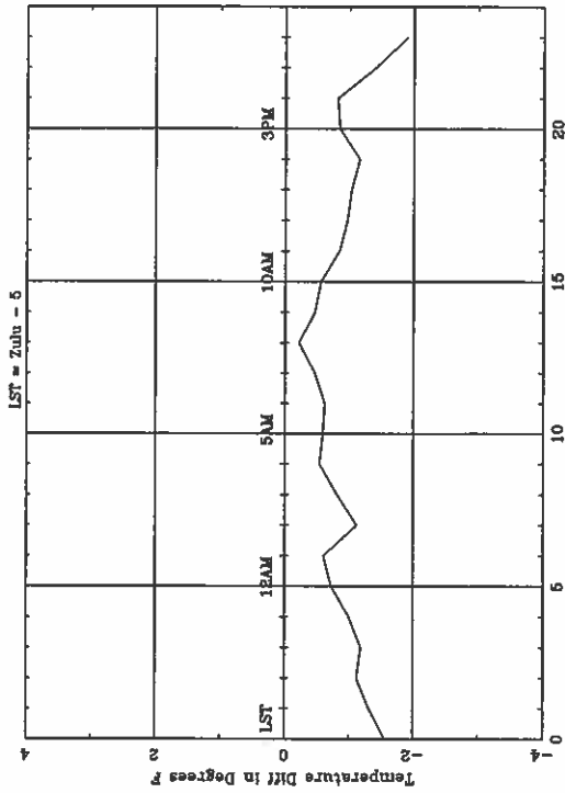
Average Diurnal Cycle for TRI - winter
