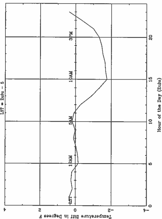
Average Diurnal Cycle for CAE - fall
