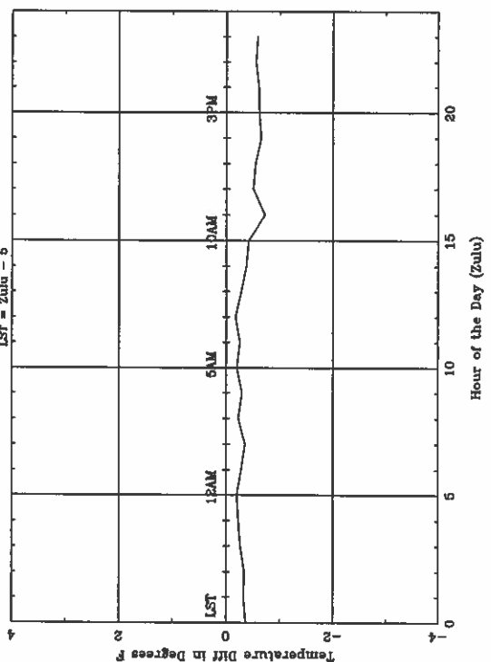
Average Diurnal Cycle for MKG - spring LST = Zulu - 5
