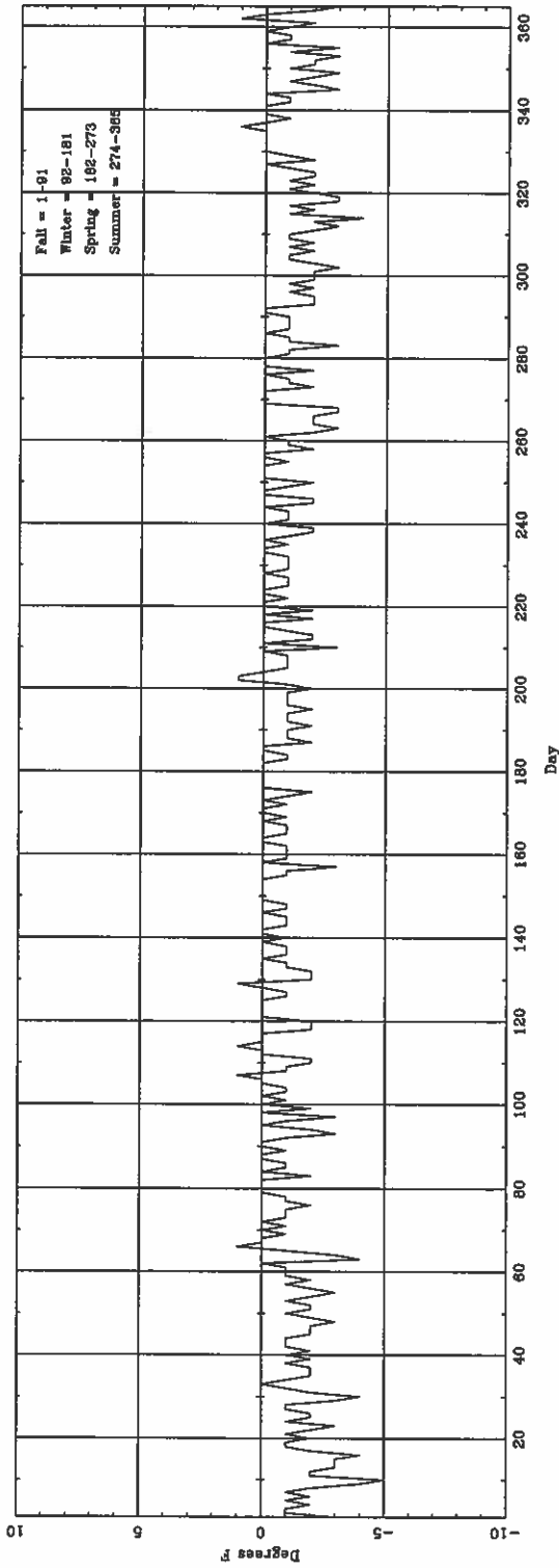
Daily AT (night hours) (ASOS - CONV) for CAE
