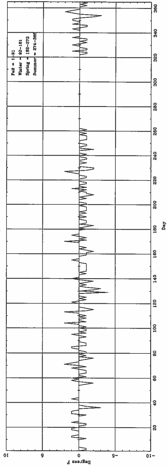
Daily \Delta T (lowest buoy) (ASOS - CONV) for APN
