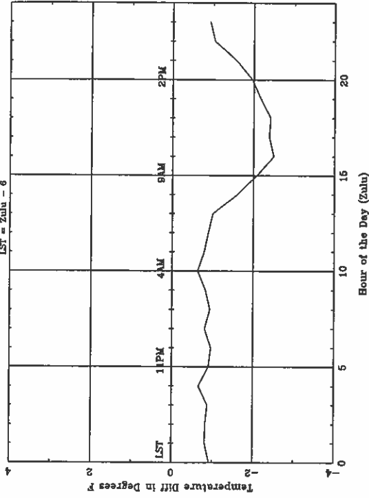
Average Diurnal Cycle for MSN - winter LST = Zulu - 6
