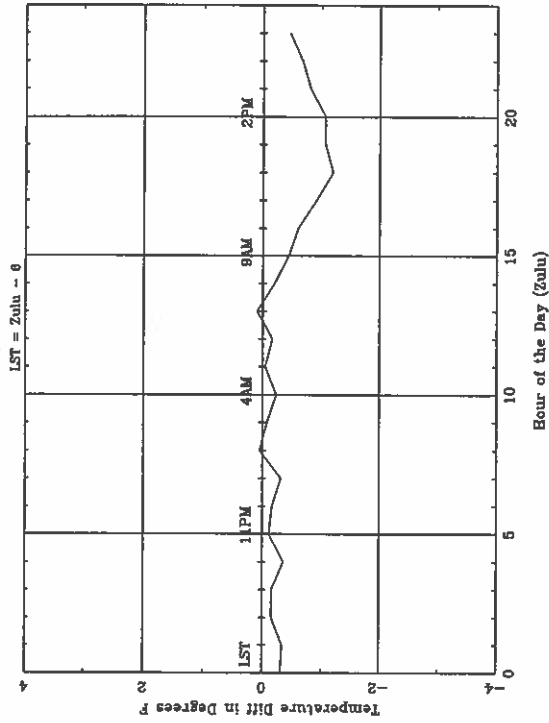
Average Diurnal Cycle for BIS - winter
