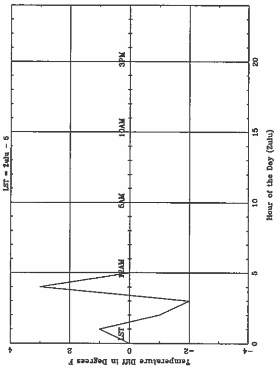
Average Diurnal Cycle for FNT - summer
