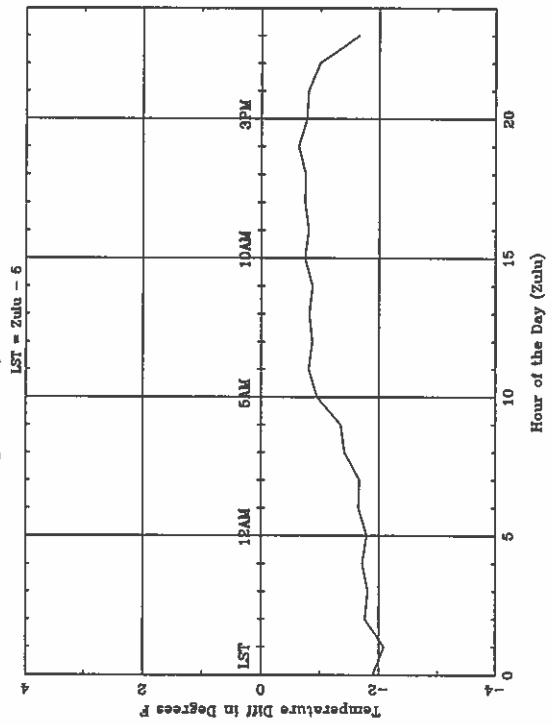
Average Diurnal Cycle for ABE - summer
