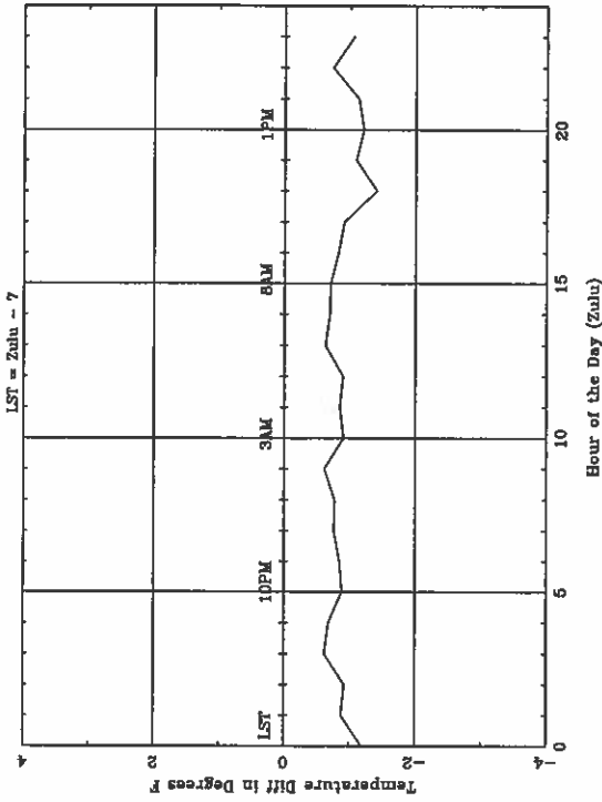
Average Diurnal Cycle for GJT - winter
