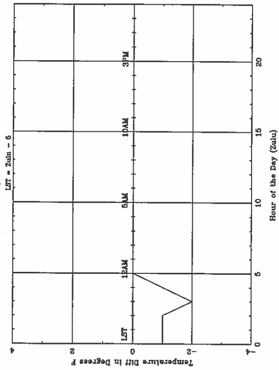
Average Diurnal Cycle for DAB - summer
