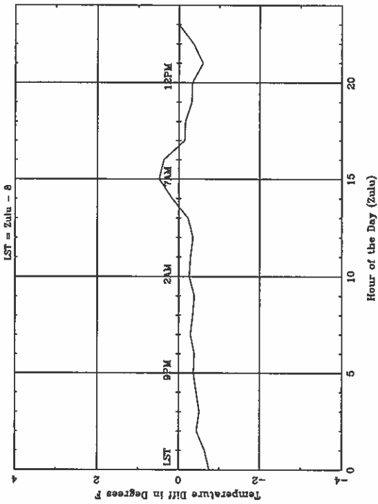
Average Diurnal Cycle for MHS - fall
