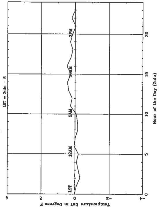
Average Diurnal Cycle for MCO - summer
