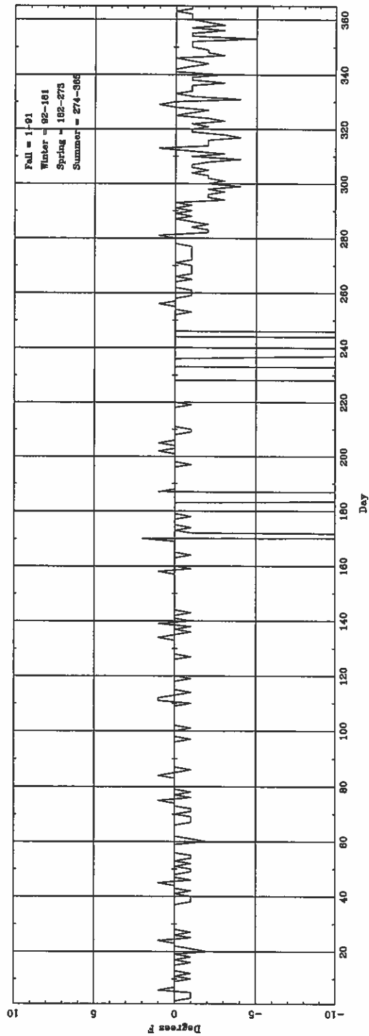
Daily \Delta T (lowest hourly) (ASOS - CONV) for MHS
