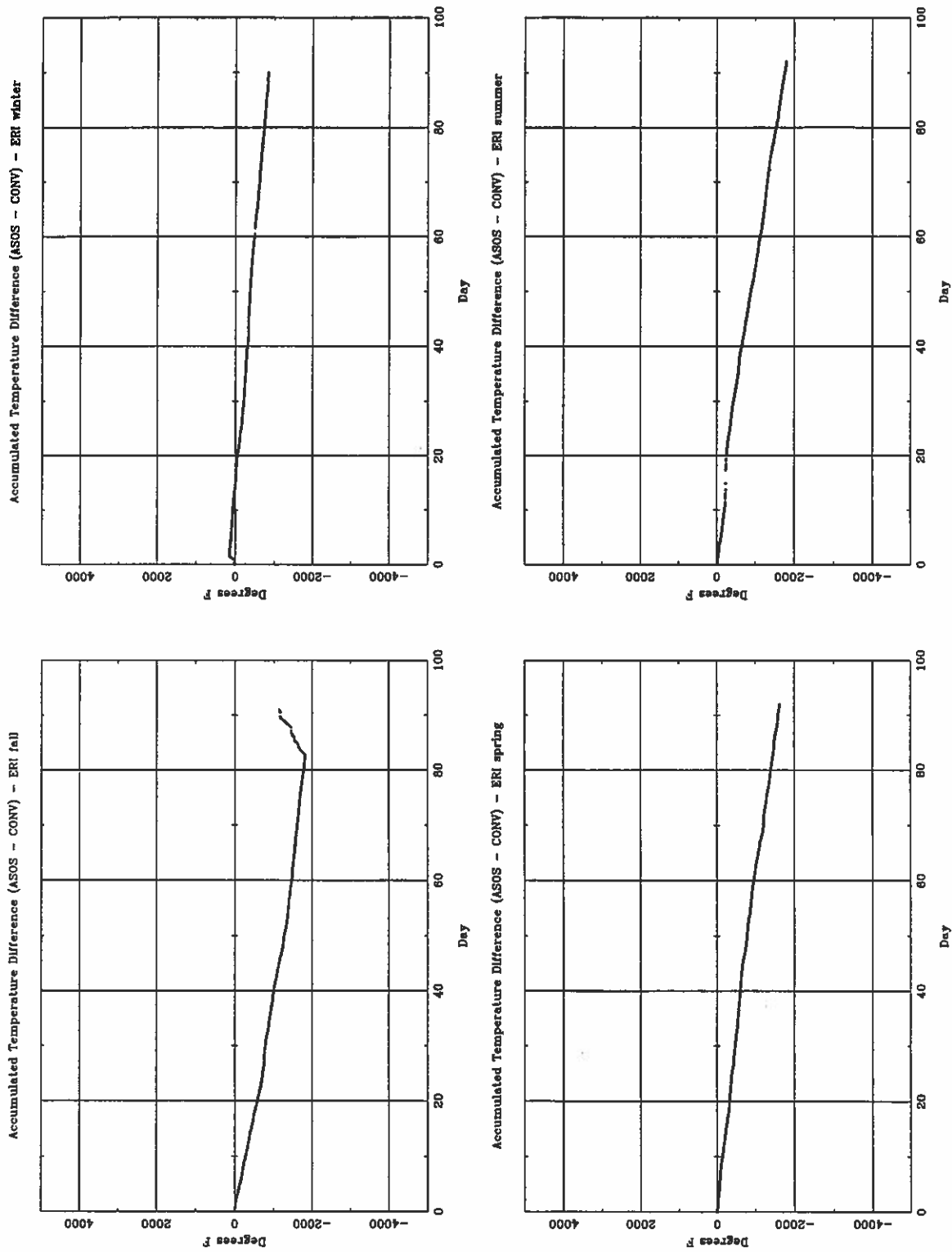
Fig. 3.1 (D) Seasonal accumulated temperature difference plots for Erie, PA.
