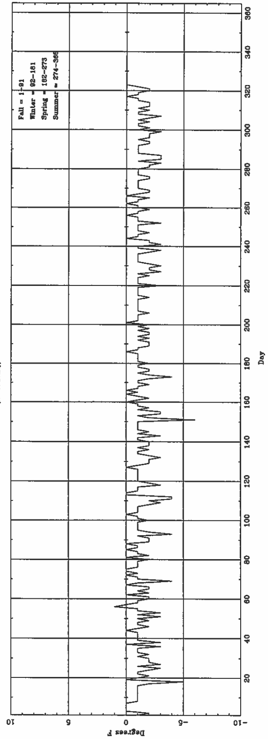
Daily \Delta T_{(lowest\ hourly)} (ASOS - CONV) for LCH
