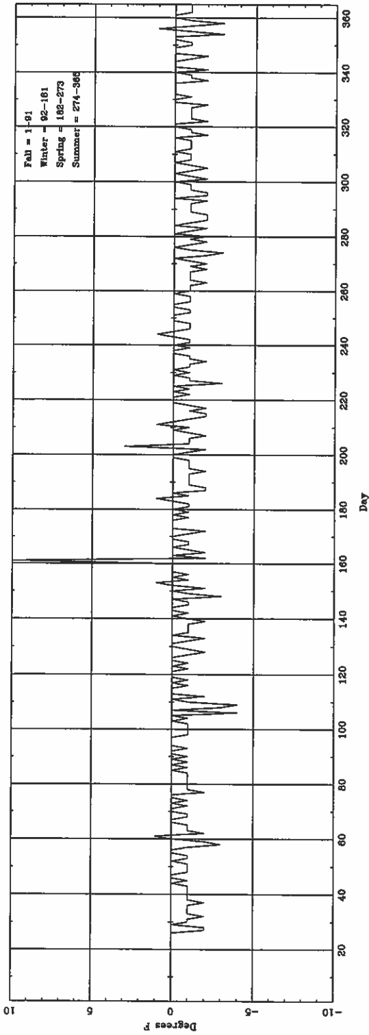
Daily AT (lightest hourly) (ASOS - CONV) for RAP
