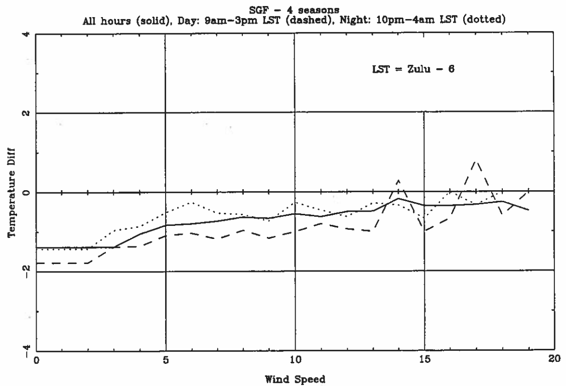
Fig. 3.3 (D) Wind speed versus temperature difference for Springfield, MO.
