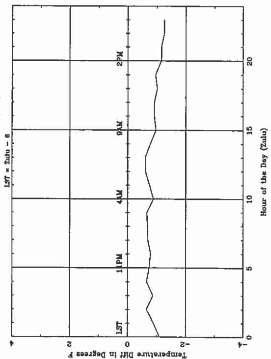
Average Diurnal Cycle for SFT - spring
