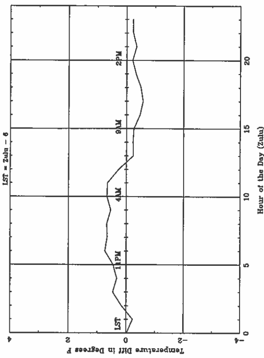
Average Diurnal Cycle for PIA - summer
