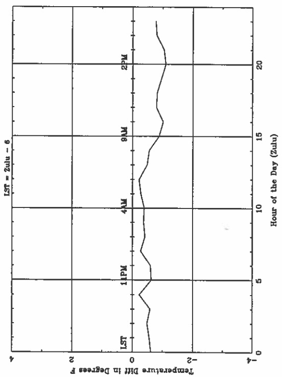
Average Diurnal Cycle for ISN - spring
