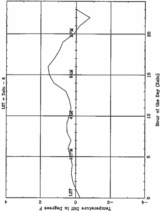
Average Diurnal Cycle for VTN - winter
