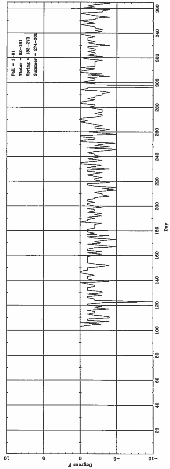
Daily \Delta T_{(\text{lowest hourly})} (ASOS - CONY) for ABE
