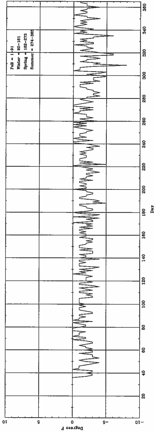
Daily AT (light hourly) (ASOS - CONV) for ABQ
