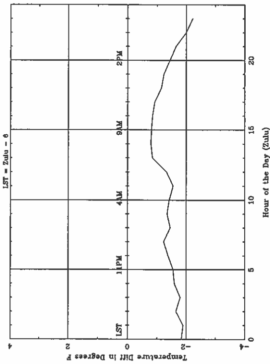
Average Diurnal Cycle for FSD - fall
