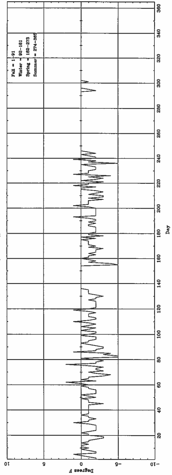
Daily \Delta T_{\text{air}}(\text{lowest hourly}) (ASOS - CONVY) for MGM
