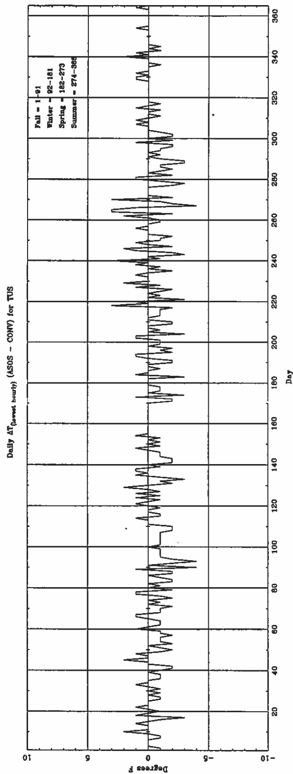
Fig. 3.2 (C) Temperature time series plots for Tucson, AZ.
