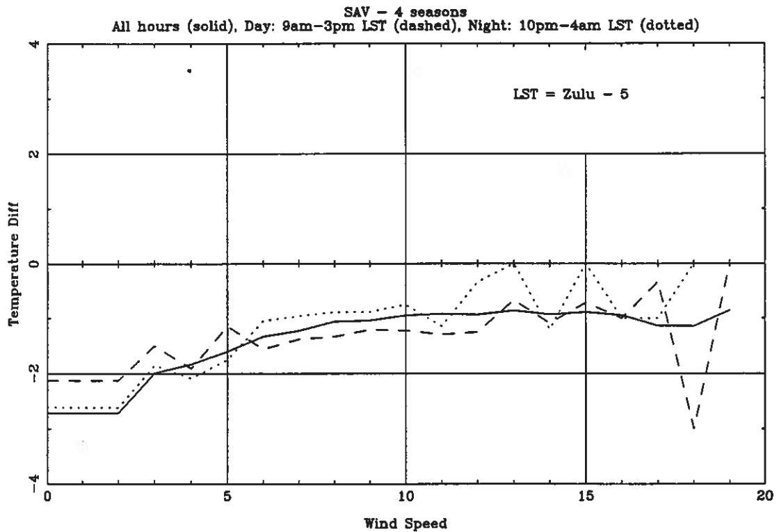
Fig. 3.3 (B) Wind speed versus temperature difference for Savannah, GA.
