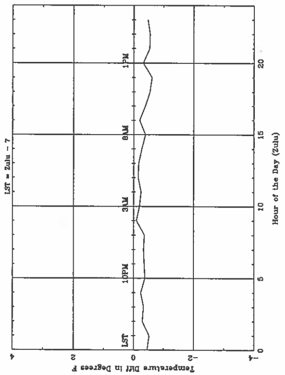
Average Diurnal Cycle for BFF - spring
