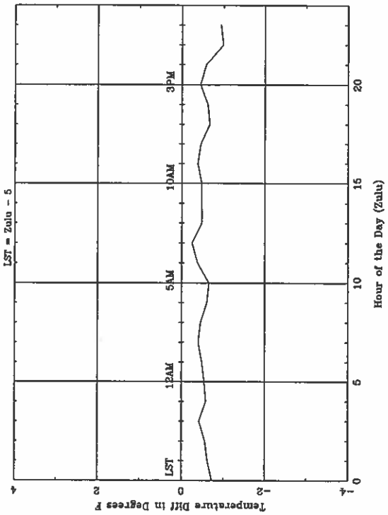
Average Diurnal Cycle for ERI - fall
