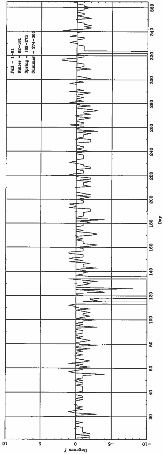
Daily \Delta T_{\text{(highest hourly)}} (ASOS - CONV) for RSL
