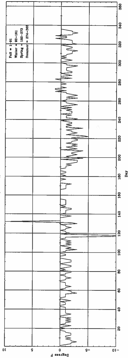
Daily \Delta T_{\text{(lightest hourly)}} (ASOS -- CONY) for PAH
