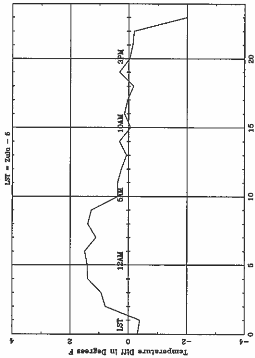
Average Diurnal Cycle for ORH - summer
