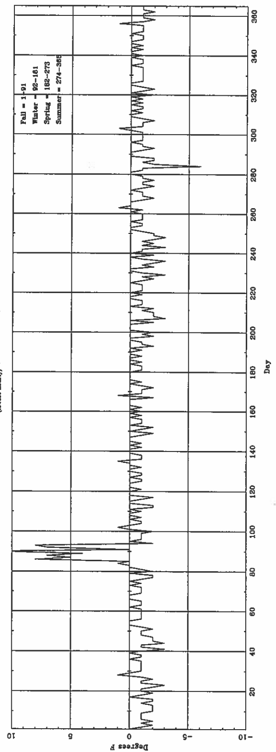
Daily \Delta T_{\text{lowest hourly}} (ASOS - CONY) for ERI
