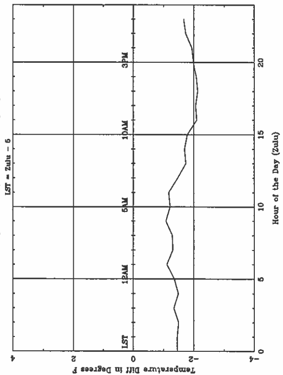
Average Diurnal Cycle for YNG - spring
