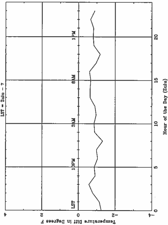
Average Diurnal Cycle for GJT - fall
