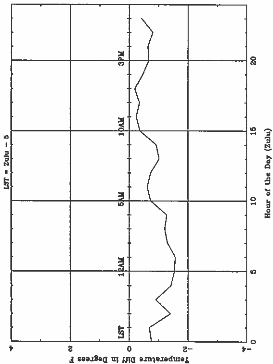
Average Diurnal Cycle for TRI - spring
