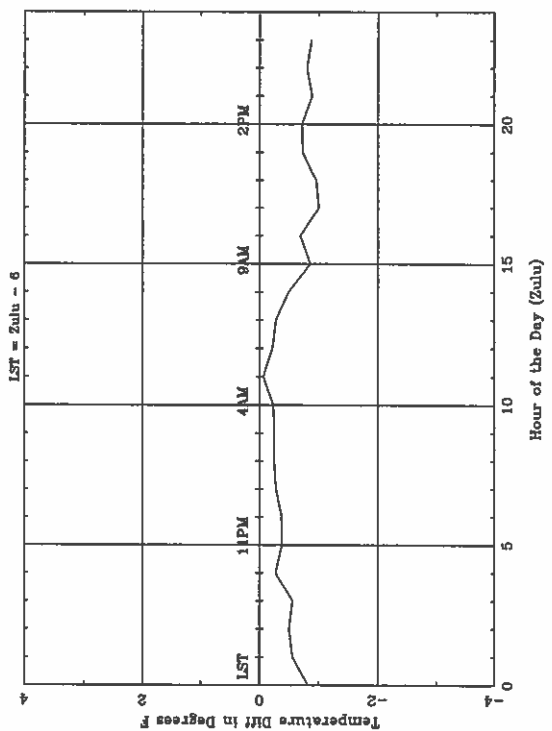
Average Diurnal Cycle for BIS - spring
