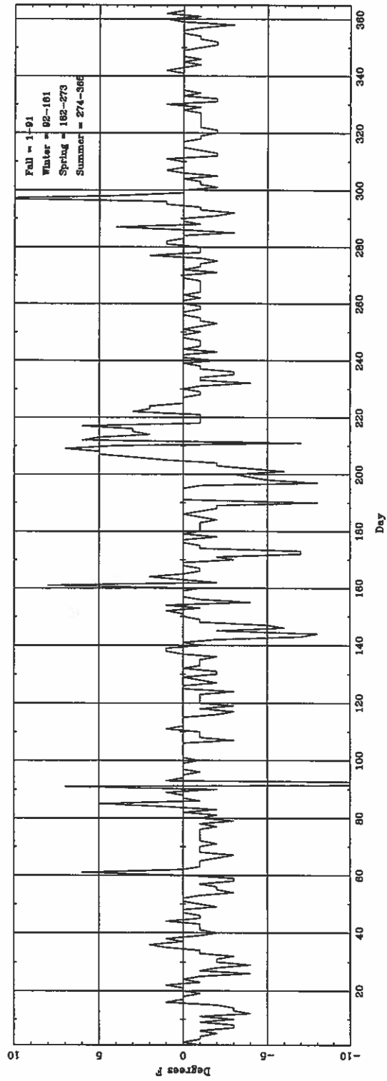
Daily \Delta T_{(forest\ beam)} (ASOS - CONV) for SGF
