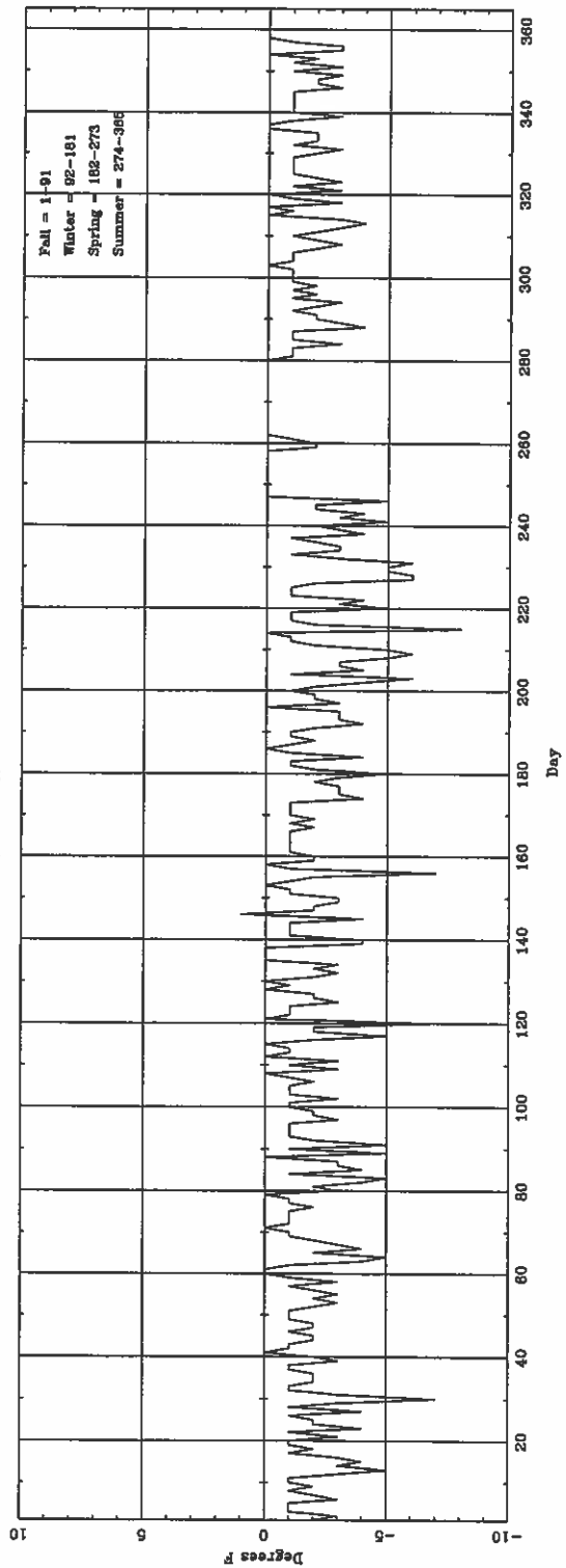
Daily \Delta T (lowest hourly) (ASOS - CONY) for SAV
