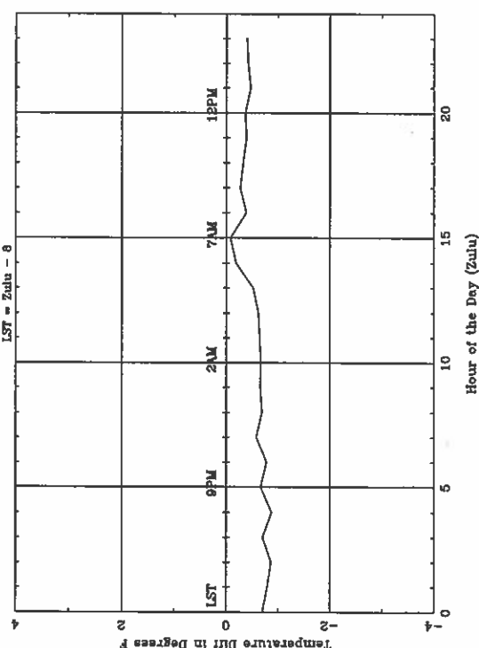
Average Diurnal Cycle for PDT -- spring LST = Zulu - 8
