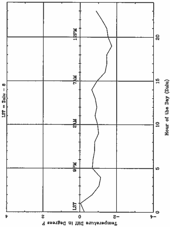
Average Diurnal Cycle for LAS - fall
