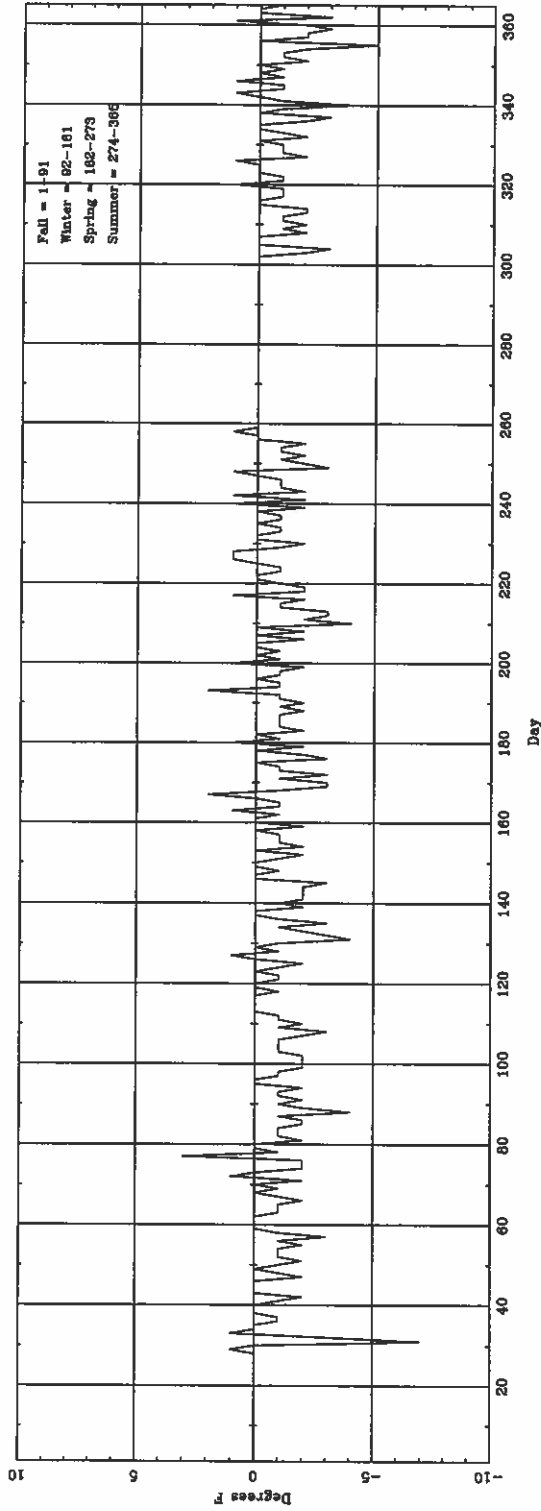
Daily \Delta T (highest hourly) (ASOS - CONV) for GJT
