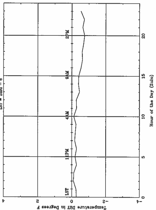
Average Diurnal Cycle for MOB - spring LST = Zulu - 6
