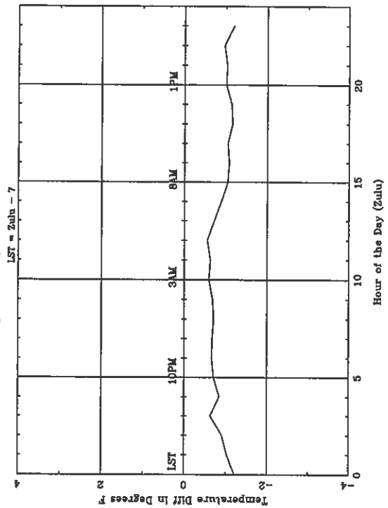
Average Diurnal Cycle for CYS - summer
