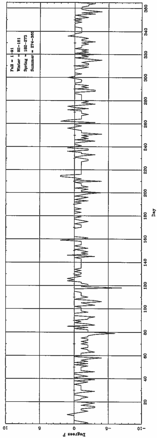
Daily \Delta T_{(darkest\ beauty)} (ASOS - CONY) for SFI
