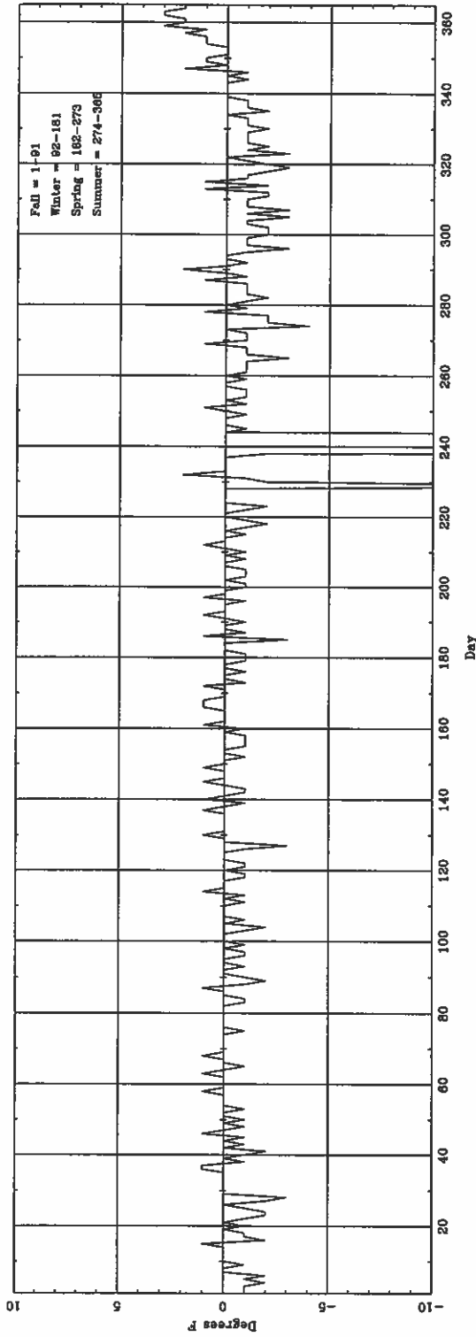
Daily \Delta T (lightest hourly) (ASOS - CONV) for MHS
