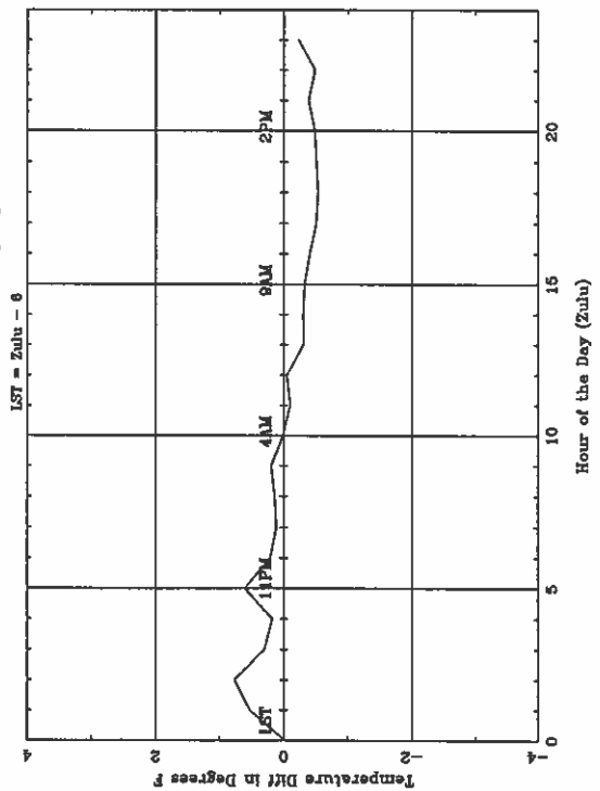
Average Diurnal Cycle for RST - spring
