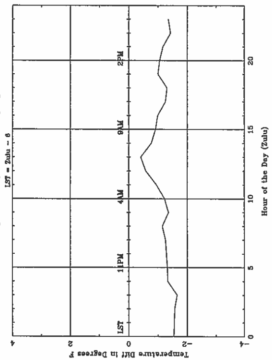
Average Diurnal Cycle for FSD - spring
