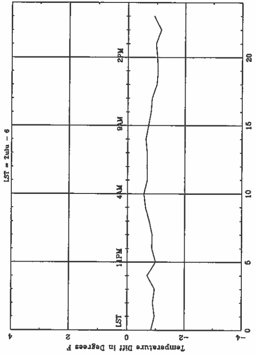
Average Diurnal Cycle for SPI - winter
