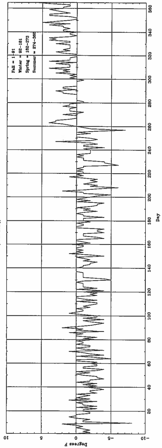
Daily \Delta T_{\text{(noct hour)}} (ASOS - CONV) for ACT
