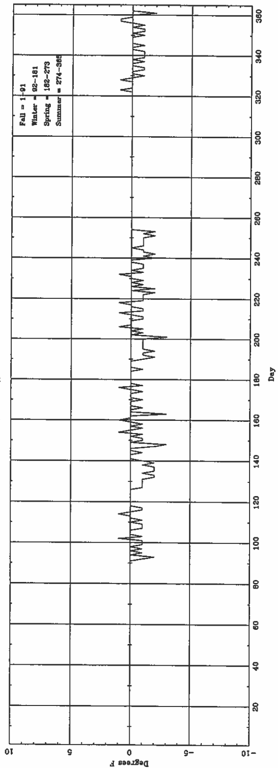
Daily \Delta T_{\text{lowest hourly}} (ASOS - CONV) for SJT
